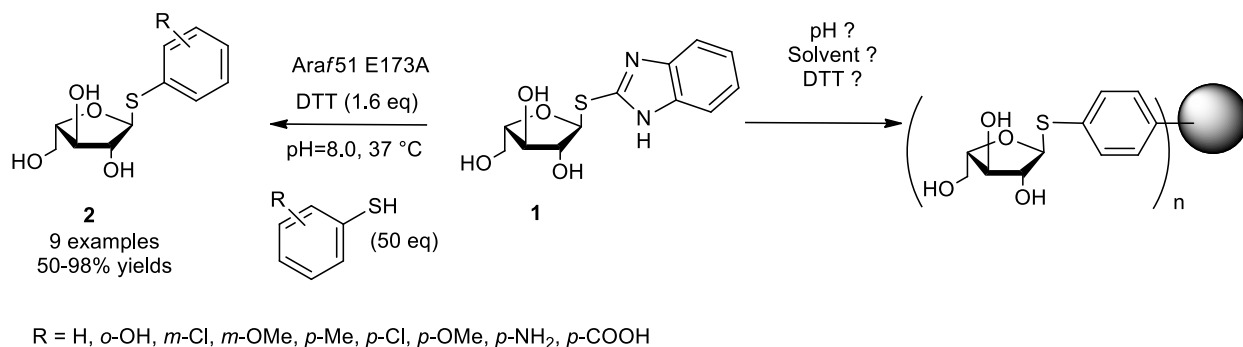
Scheme 1. Biocatalyzed synthesis of various thioaryl furanosides.
