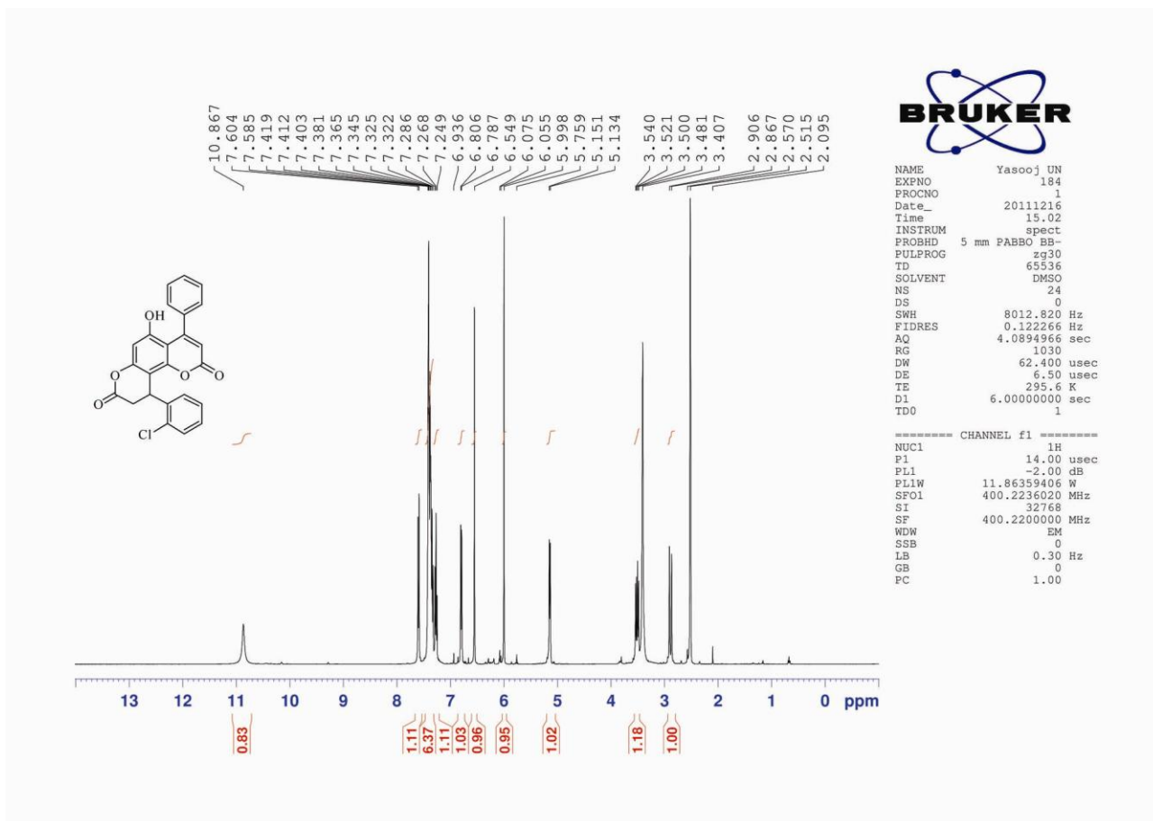
1 H NMR spectrum of compound 8f
