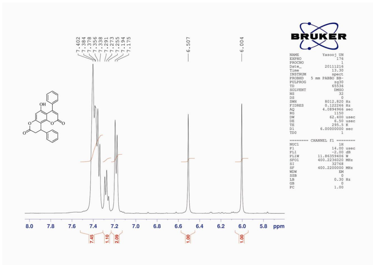
1 H NMR (expanded) spectrum of compound 8e
