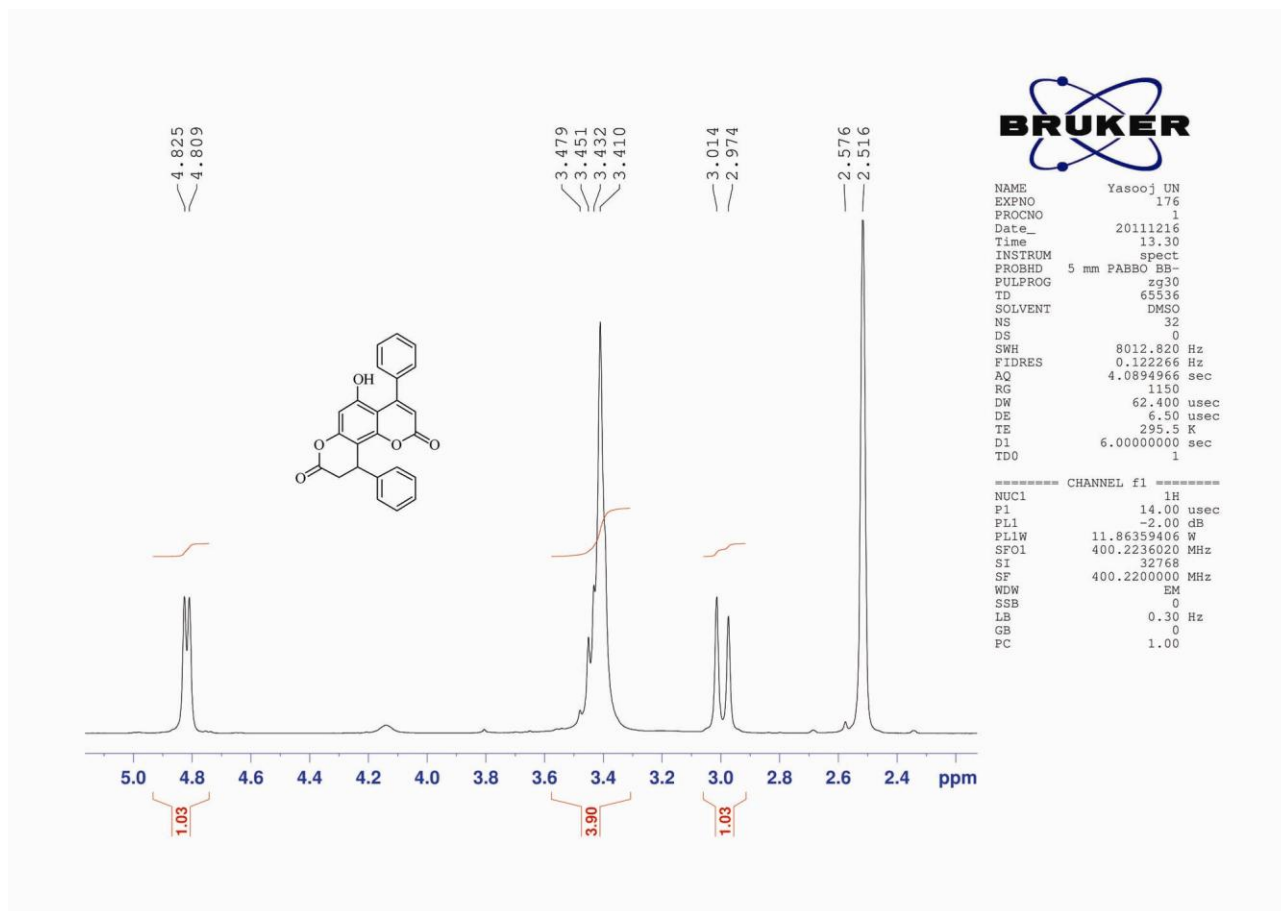
^1\text{H} NMR (expanded) spectrum of compound 8e
