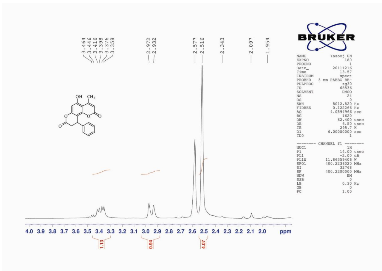
1 H NMR (expanded) spectrum of compound 8a
