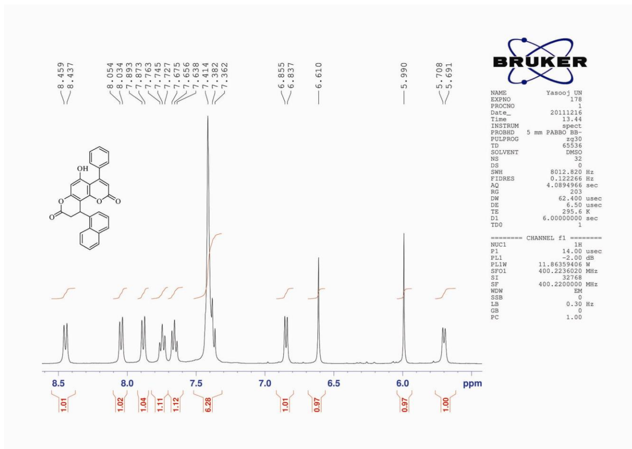
1 H NMR (expanded) spectrum of compound 8h
