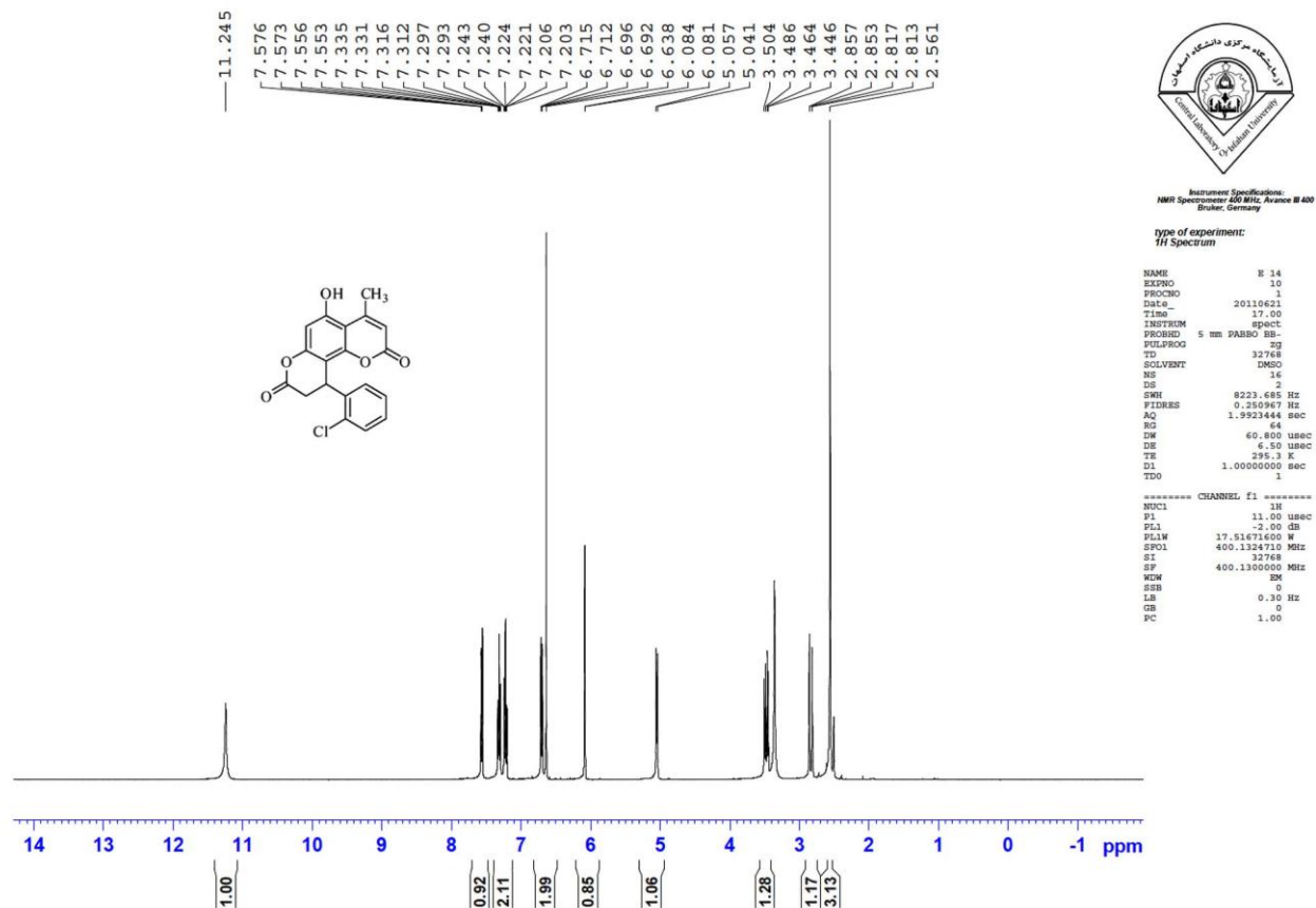
^1\text{H} NMR spectrum of compound 8b
