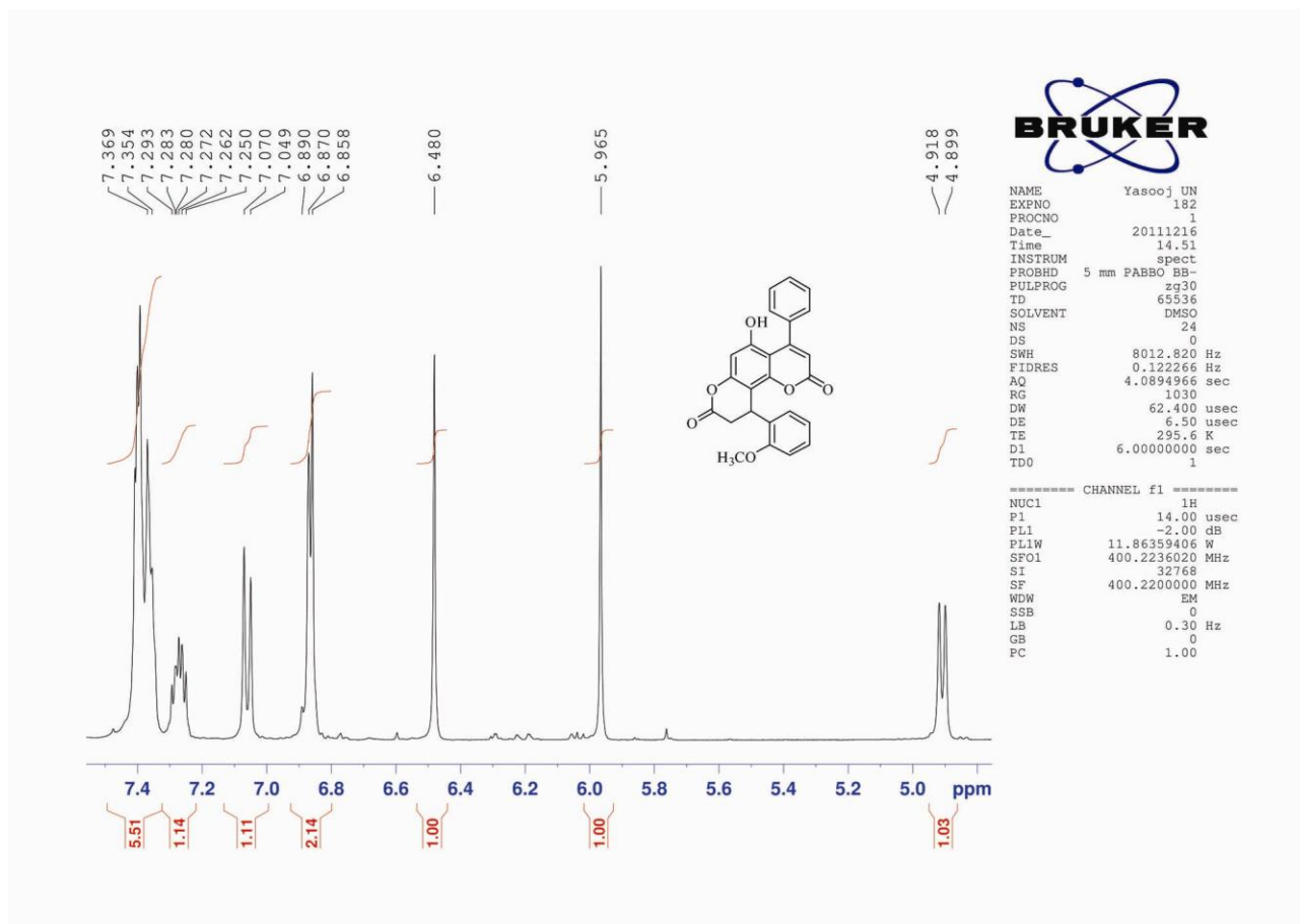
1 H NMR (expanded) spectrum of compound 8g
