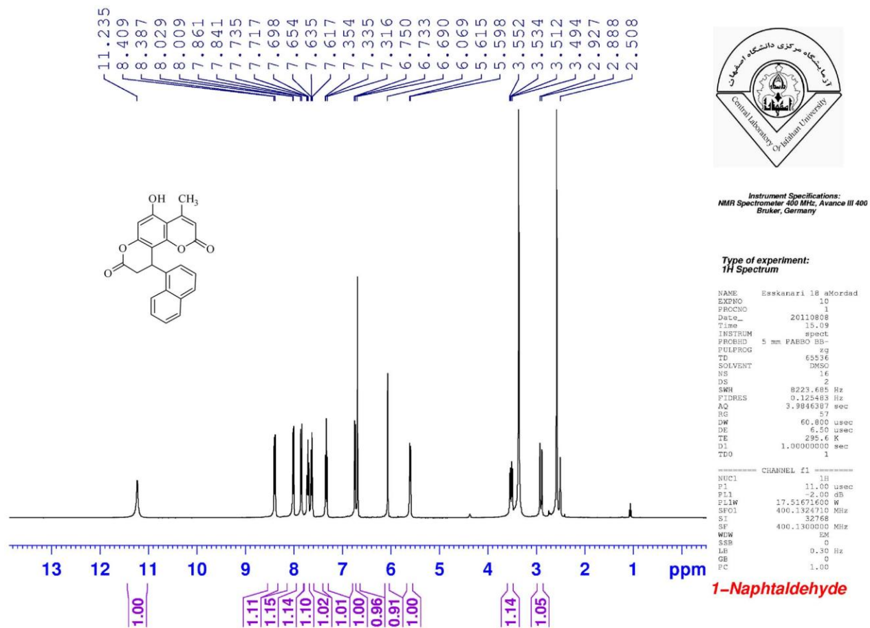
1 H NMR spectrum of compound 8d
