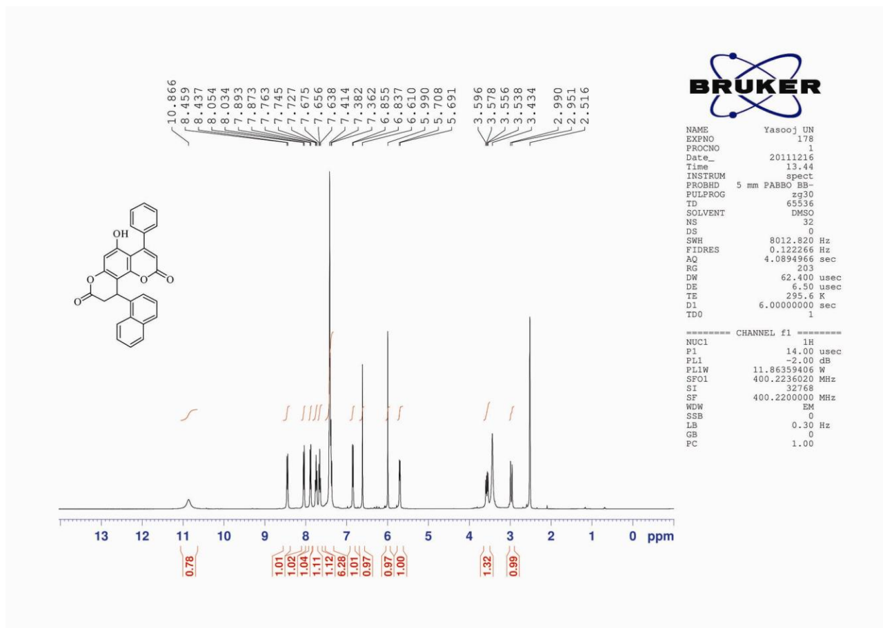
1 H NMR spectrum of compound 8h
