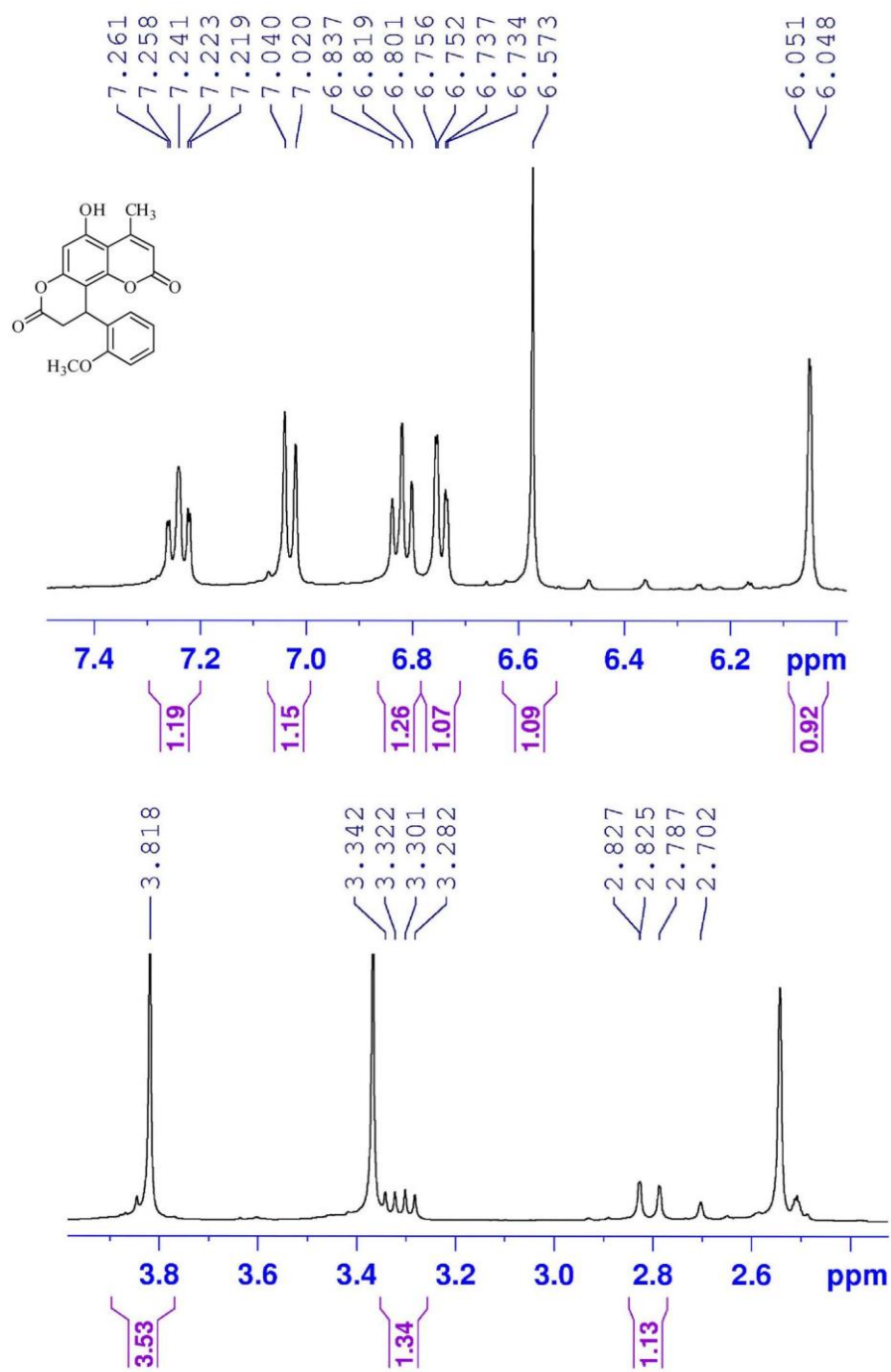
1 H NMR (expanded) spectrum of compound 8c
