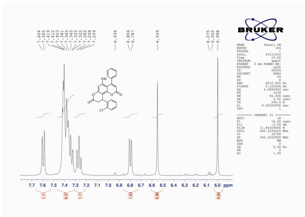
^1\text{H} NMR (expanded) spectrum of compound 8f
