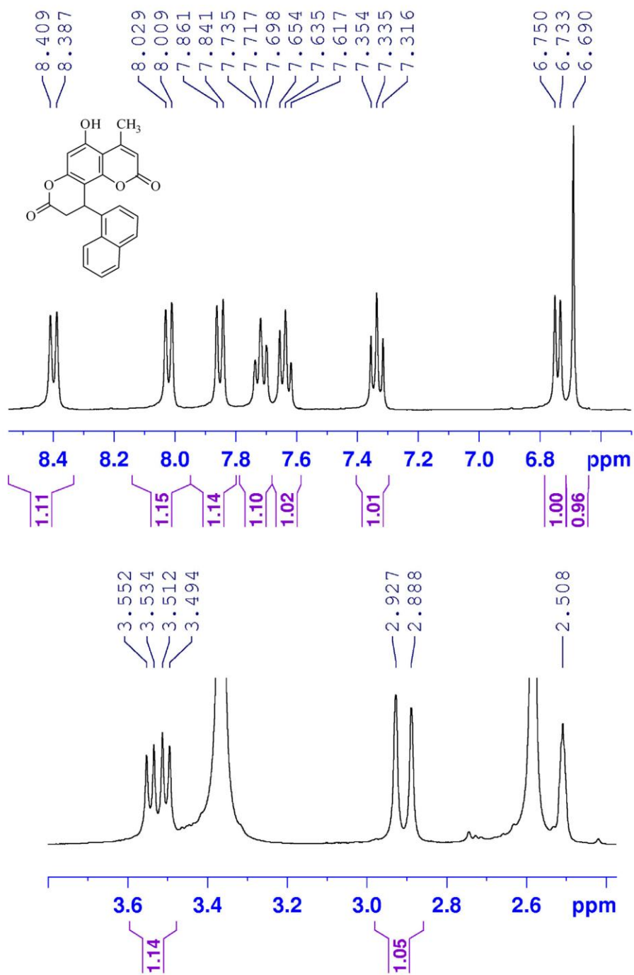
1 H NMR (expanded) spectrum of compound 8d
