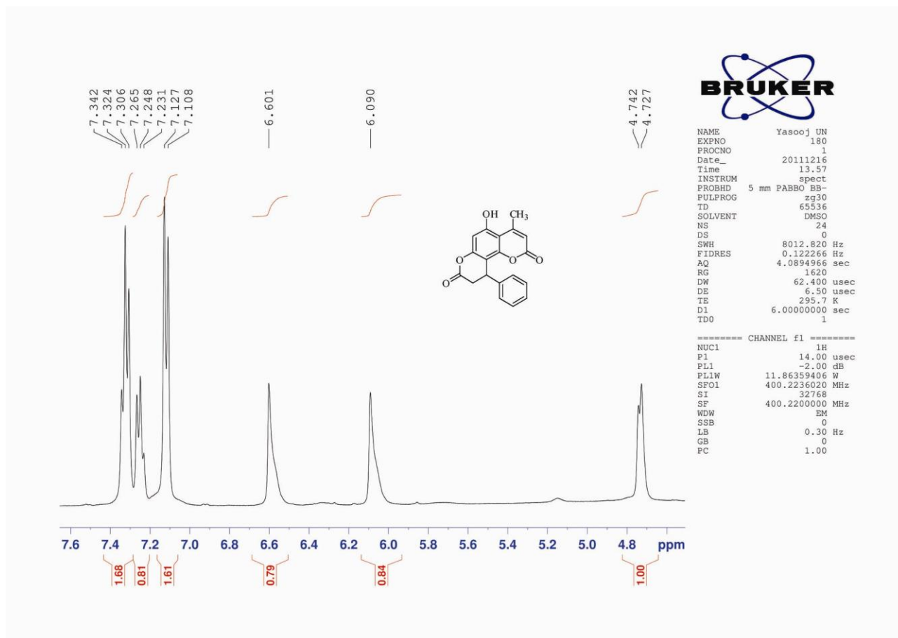
^1\text{H} NMR (expanded) spectrum of compound 8a
