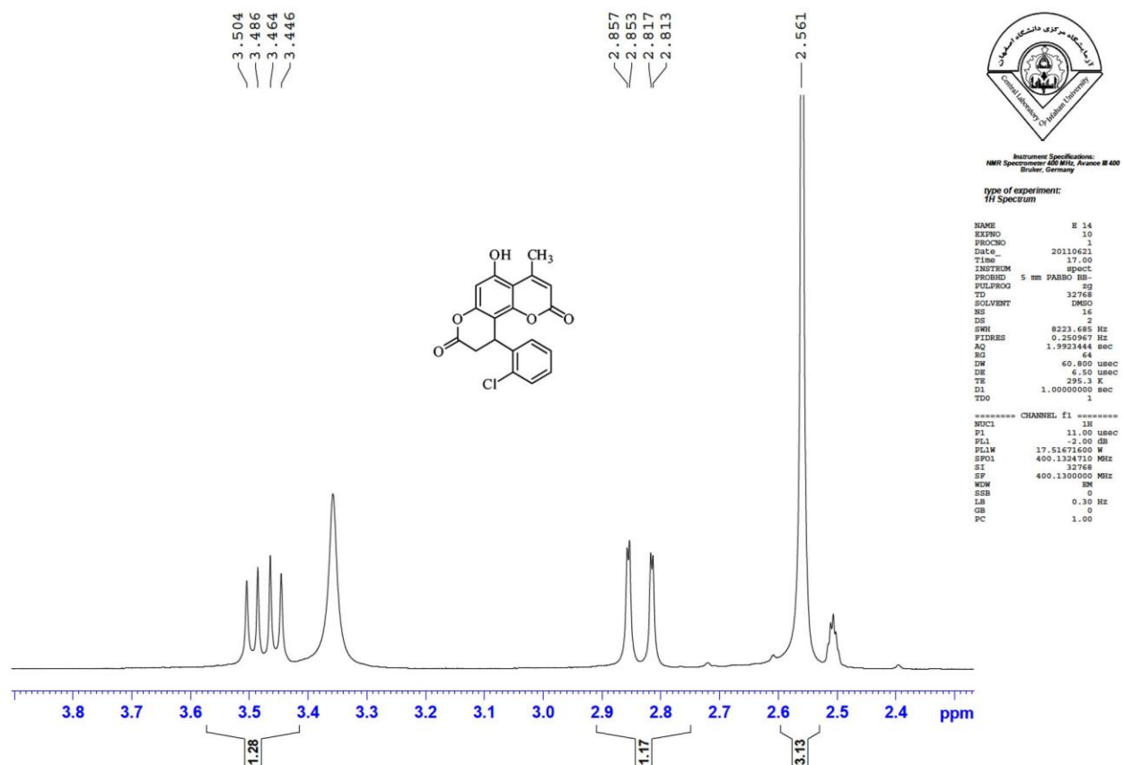
^1\text{H} NMR (expanded) spectrum of compound 8b
