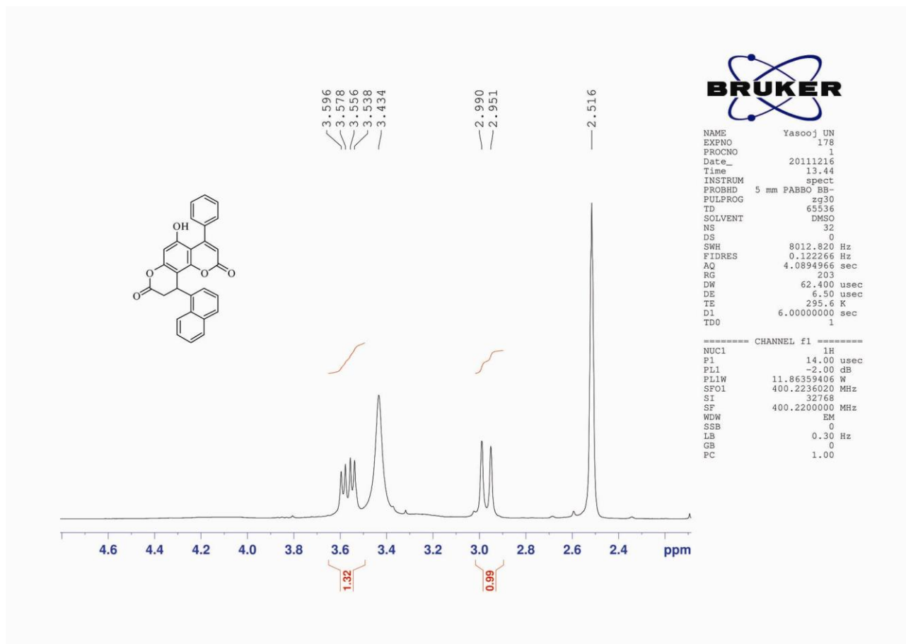
^1\text{H} NMR (expanded) spectrum of compound 8h
