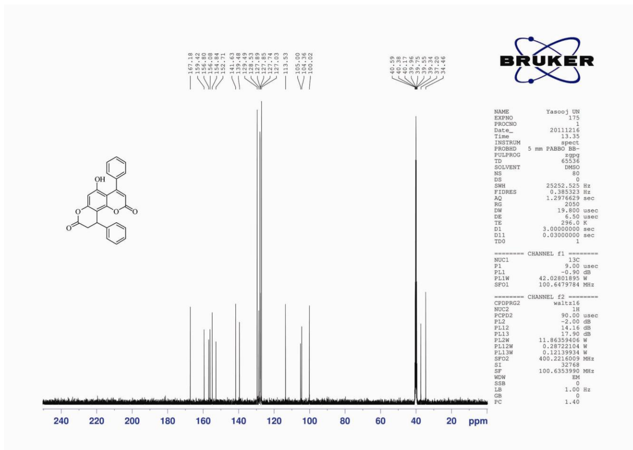
^{13}\text{C} NMR spectrum of compound 8e
