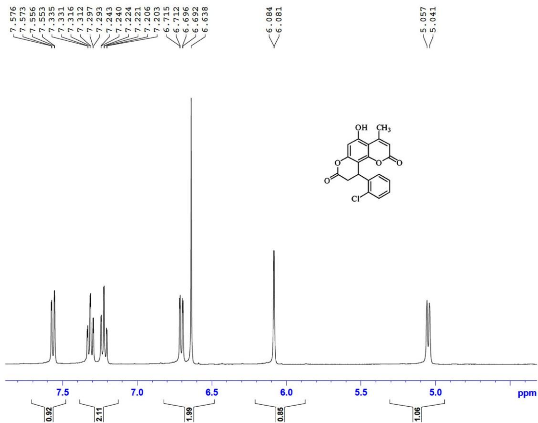
1 H NMR (expanded) spectrum of compound 8b
