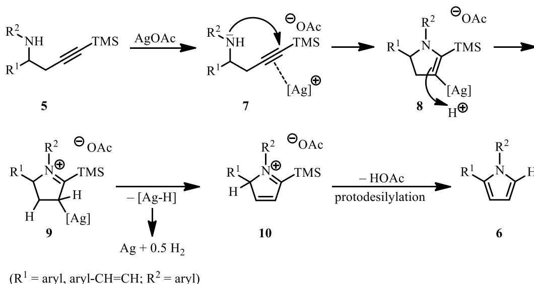
Scheme 2. Proposed mechanism for the silver(I)-promoted oxidative cyclization of homopropargylamines 5 .
