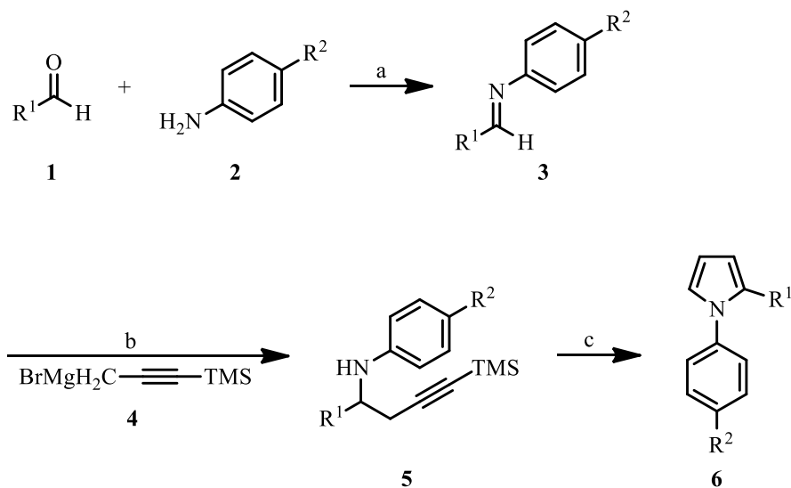
Scheme 1. Synthesis of pyrroles 6a–c . Reagents and conditions: (a) MgSO 4 , EtOAc, r.t., 1–2 h; (b) BF 3 ·Et 2 O, THF, –23 °C, 30 min; then: 4 in Et 2 O, –23 °C 15 h; (c) 1.1 equiv AgOAc, CH 2 Cl 2 , r.t., 4 d.
