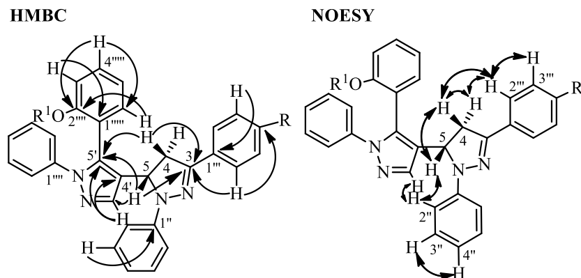
Figure 3. Main correlations observed in the HMBC and NOESY spectra of both diastereomers of pyrazolyl-2-pyrazolines 2a-g and 3a-c,e .
