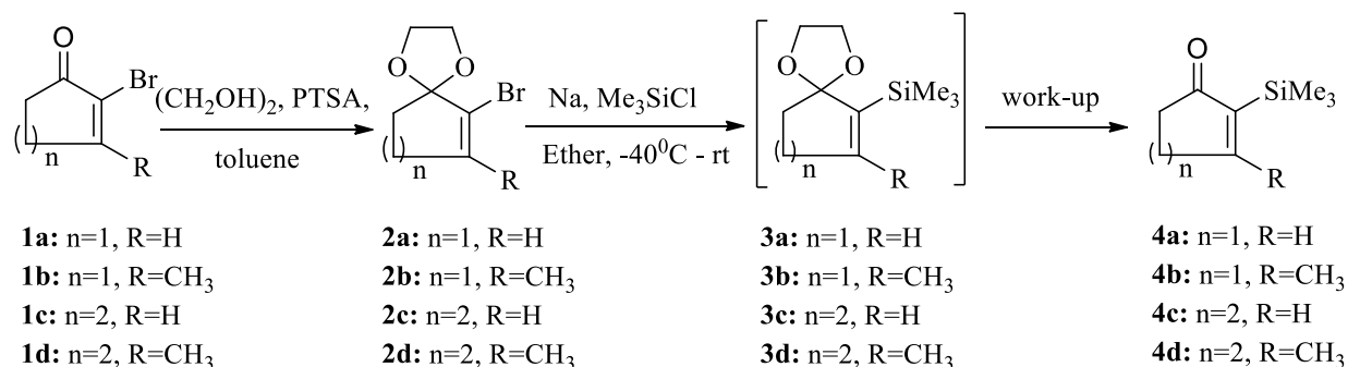
Scheme 1. Synthesis of some 2-trimethylsilylcycloalkenones.
