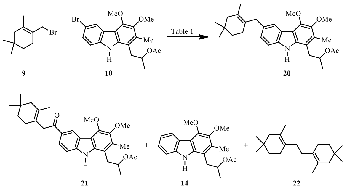
Scheme 5. Synthesis of 6-( \beta -cyclolavandulyl)carbazole 20 .
