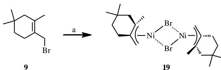
Scheme 4. Synthesis of the dimeric \pi -( \beta -cyclolavandulyl)nickel bromide complex 19 . Reagents and conditions: (a) excess of \text{Ni}(\text{CO})_4 , benzene, 60–65 °C, 2.5–3.5 h.
