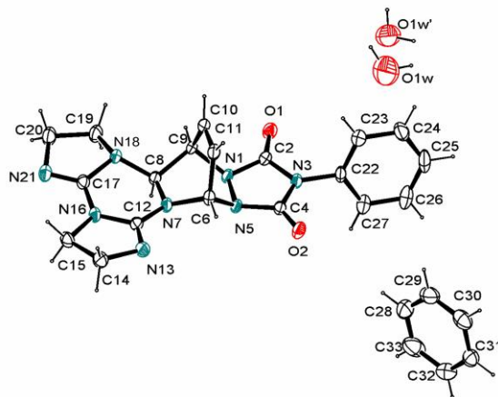
Figure 1. X-Ray structure of compound 6 showing atomic labels and displacement ellipsoids at the 50% probability level.
