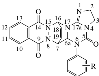
Figure 5. Numbering of atoms used to describe ^1\text{H} and ^{13}\text{C} NMR spectra of compounds 11a–b .
