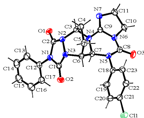
Figure 3. X-Ray structure of compound 9b showing atomic labels and displacement ellipsoids at the 50% probability level.
