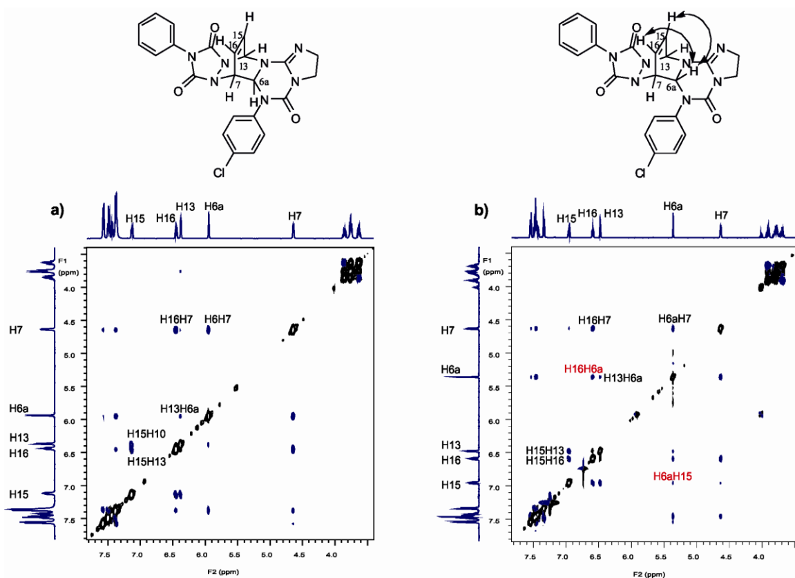
Figure 2. a) The ROESY spectrum and the proposed structure of the higher-yield stereoisomer of compound 7e . b) The ROESY spectrum and the proposed structure of the lower-yield stereoisomer of compound 7e . The diagnostic cross-peaks are highlighted red.
