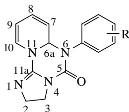
Figure 4. Numbering of atoms used to describe 1 H and 13 C NMR spectra of compounds 3b–d and 3g .
