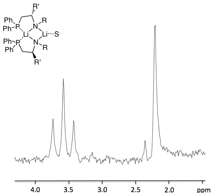
Figure 4. 6 Li NMR spectrum of (Li-2) 2 (0.3 M) obtained at -78 °C in Et 2 O solution.
