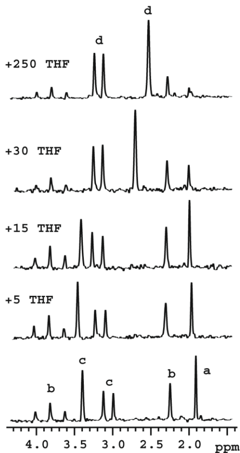
Figure 7. The equilibrium between (Li-2) 2 , (n-BuLi) 4 , and mixed complexes n-BuLi/(Li-2), R= R'= i-Pr.
