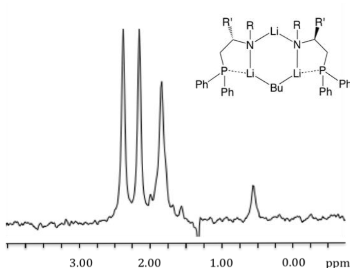
Figure 1. 6 Li NMR of Li-1 and n -BuLi in toluene solution, along with the proposed mixed complex that forms in solution (R= i -Pr and R'=Ph). The minor peak at 0.45 ppm is due to an unassigned lithium signal, possibly arising from a larger aggregate of the amide.
