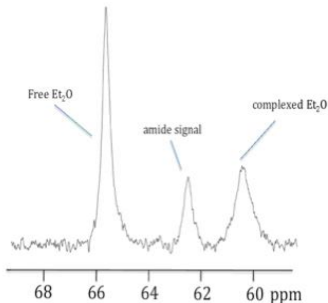
Figure 5. A Selected region (the \text{CH}_2 carbons of \text{Et}_2\text{O} ) of the ^{13}\text{C} NMR spectra with approx. 2 equivalents of \text{Et}_2\text{O} added to the toluene- d_8 solution of Li-1. Both free uncoordinated and coordinated \text{Et}_2\text{O} ether signals appear as separate signals due to slow ethereal ligand exchange on the NMR time scale -80\text{ }^\circ\text{C} .
