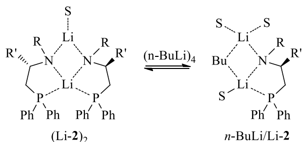
Figure 7. The equilibrium between (Li-2) 2 , (n-BuLi) 4 , and mixed complexes n-BuLi/(Li-2), R= R'= i-Pr.
