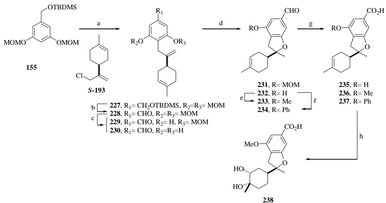
Scheme 19. Reagents and conditions: a) n BuLi, TMEDA, CuI, S-193 (82%); b) 1. TBAF, THF; 2. PCC, CH 2 Cl 2 (90%, overall); c) 3N HCl, 2-PrOH, rt, 8h ( 229 , 21%; 230 , 52%); d) Amberlyst-15, CH 2 Cl 2 , rt; e) CH 3 I, Ag 2 O, CHCl 3 (95%); f) Ph 3 Bi(OAc) 2 , Cu 0 , CH 2 Cl 2 (75%); g) AgNO 3 , KOH, EtOH, H 2 O ( 235 , 63%); h) OsO 4 , Me 3 NO·2H 2 O, t BuOH (68%).
