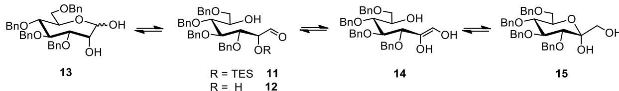
Figure 2. Equilibria available to hydroxy-aldehydes.
