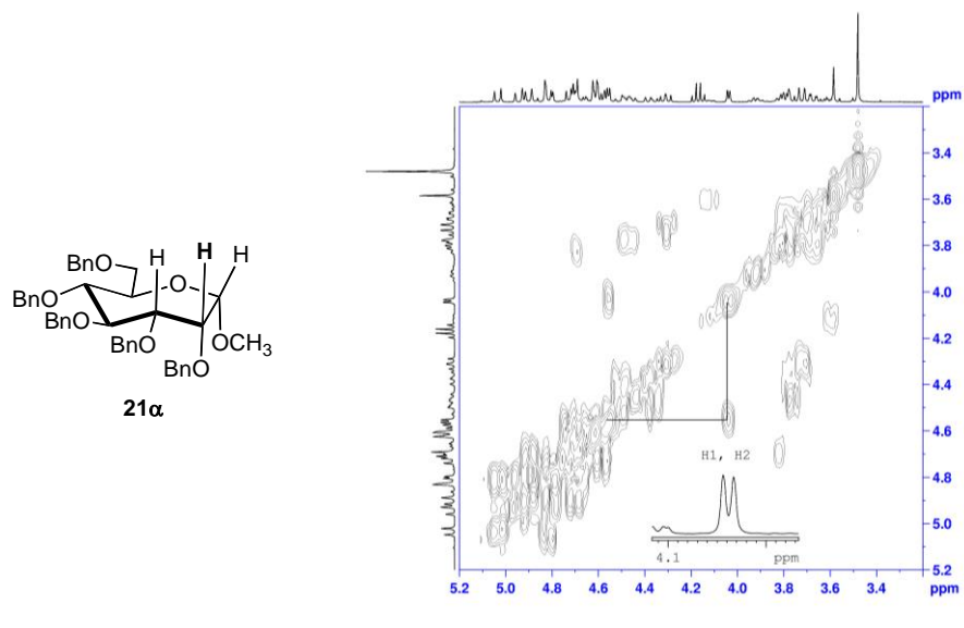
Figure 3. H2 as a diagnostic for determining the stereochemistry of the C2 hydroxyl group of 21α . Left is the structure assigned to 21α ; on the right is a detail of a COSY spectrum of 21 with inset showing signal for H2.
