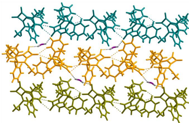
Figure 5. Hydrogen-bonding 2D network linked through the water molecule. Hydrogen bonds are represented by dashed lines.
