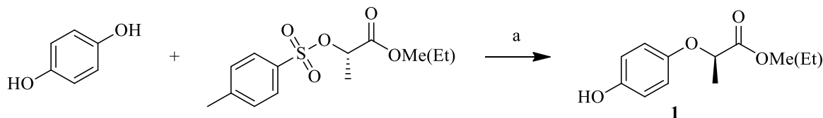
Scheme 1. Reagents and conditions: (a) NaOH, MeOH, 40 °C; HCl acid.
