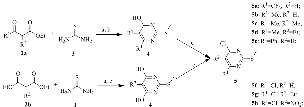
Scheme 2. Reagents and conditions: (a) NaOMe, MeOH, reflux; (b) SO 2 (OMe) 2 , NaOH, H 2 O,
