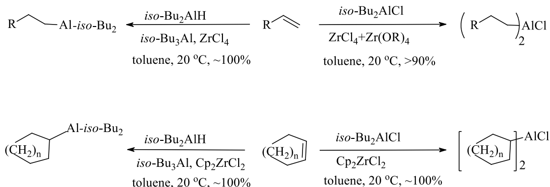
Scheme 15. The efficient methods for hydroalumination of cyclic and acyclic olefins.
