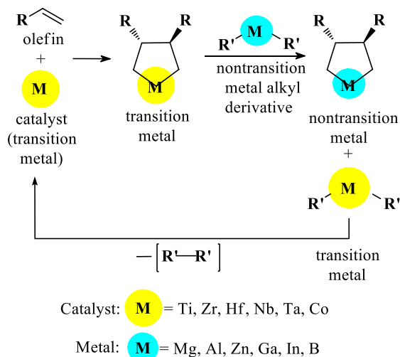
Scheme 16. Catalytic replacement of transition metal atoms in metallacarbycles by the atoms of nontransition metals.
