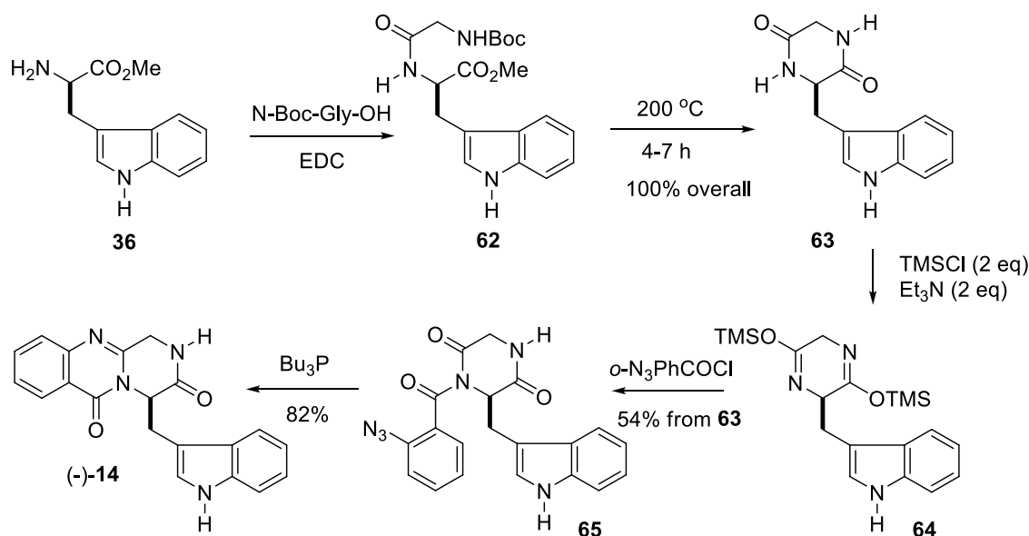
Scheme 8. Avendaño synthesis of (-)-glyantrypine 14 en route to alantrypinone.
