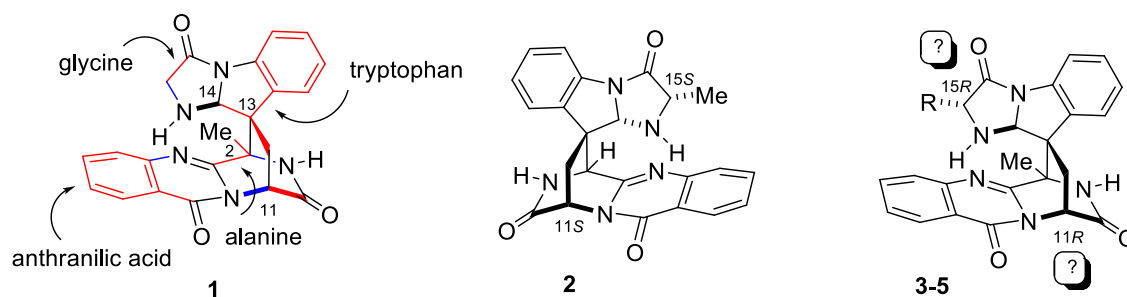
Figure 7. Proposed biosynthetic origins of spiroquinazoline 1 [carbon skeleton in red and \alpha -amino bonds in blue] and lapatin A 2 , and stereochemical questions associated with alkaloids 3–5 .
