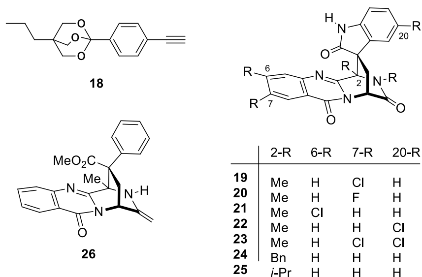
Figure 9. Synthetic inhibitors of EBOB 18 binding to housefly head membranes.
