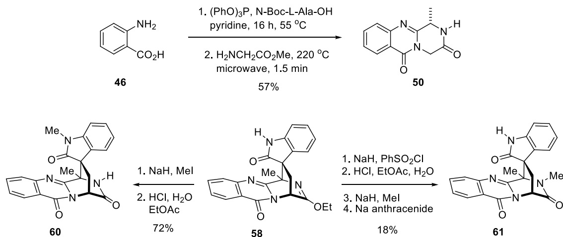
Scheme 7. Tactical improvements on the Kende synthesis and lactam differentiation.
