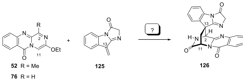
Scheme 22. A possible variation on the Diels-Alder theme.
