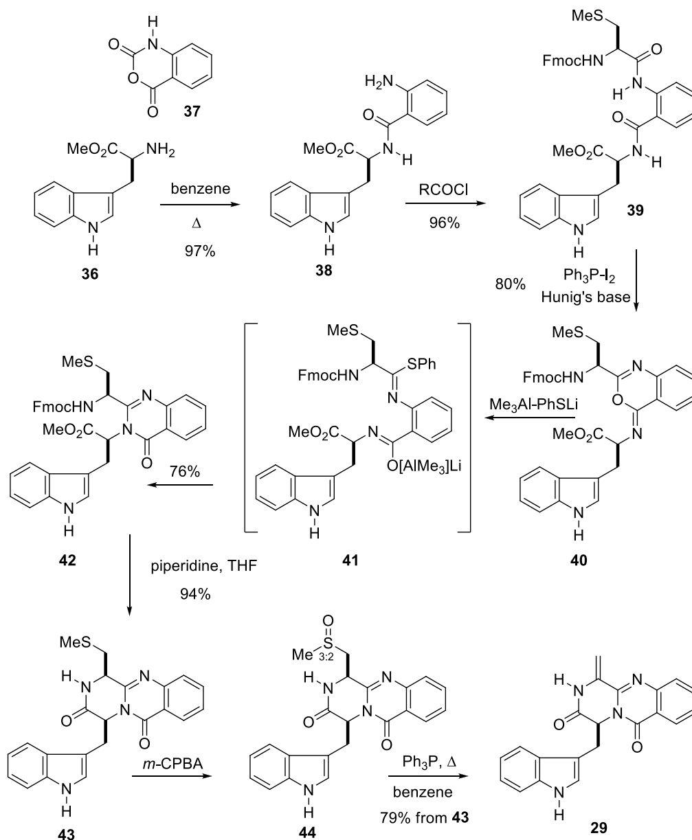
Scheme 3. Preparation of enamide 29 en route to ent -alantrypinone.
