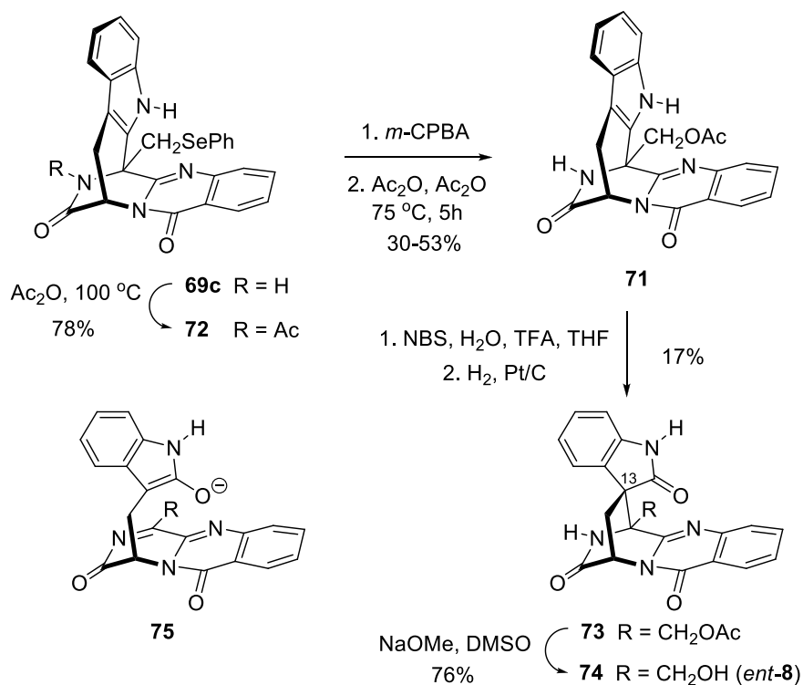
Scheme 11. Completion of ent -serantrypinone synthesis ( 74 = ent -8).
