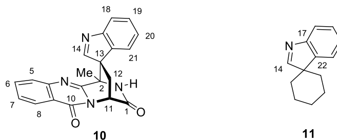
Figure 5. Structure proposed for alantrypinene B 10 and model 11 for NMR analyses.
