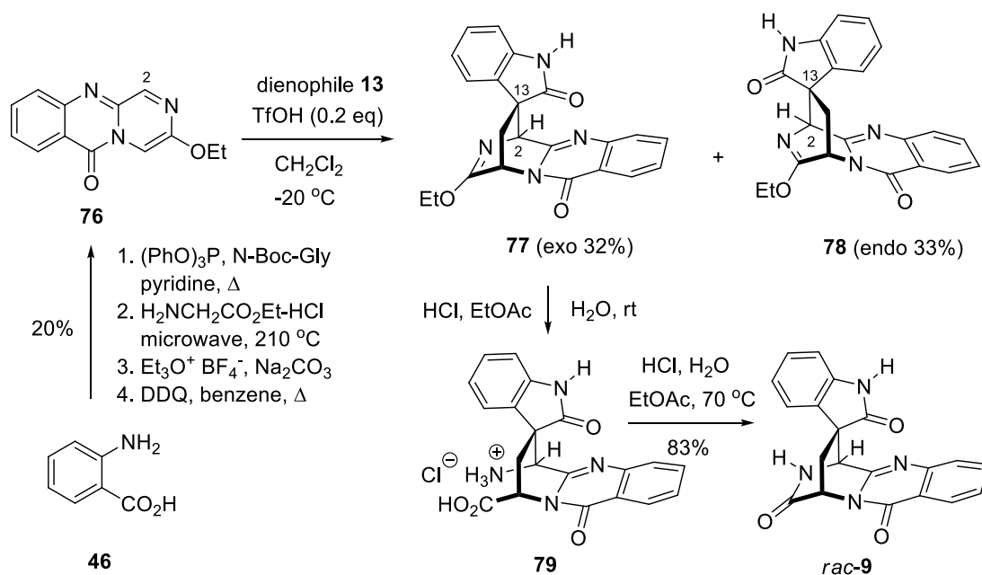
Scheme 12. Syngenta synthesis of racemic lapatin B ( rac - 9 ).
