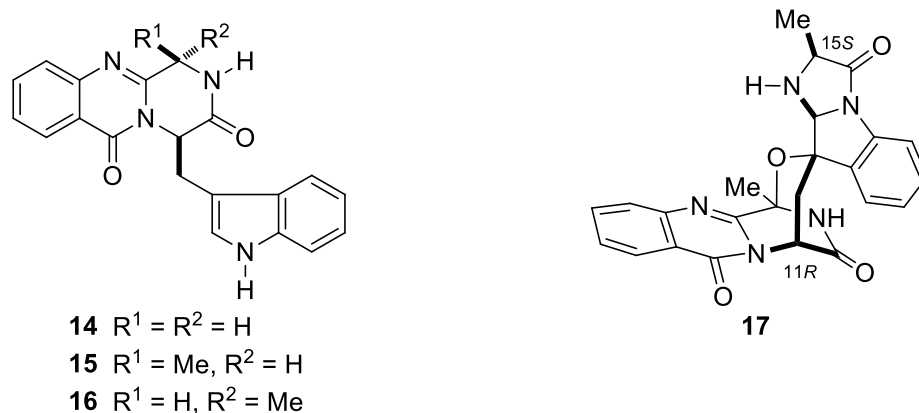
Figure 8. Structures of gyantrypine 14 and fumiquinazolines G 15 , F 16 and C 17 .
