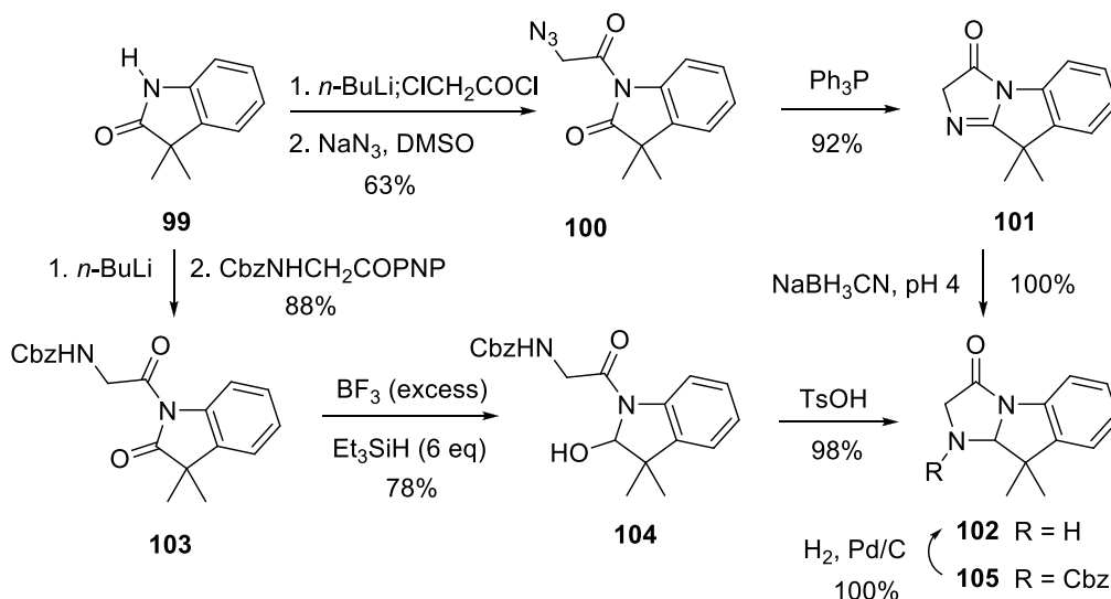
Scheme 17. Model studies for conversion of alantrypinone to spiroquinazoline.
