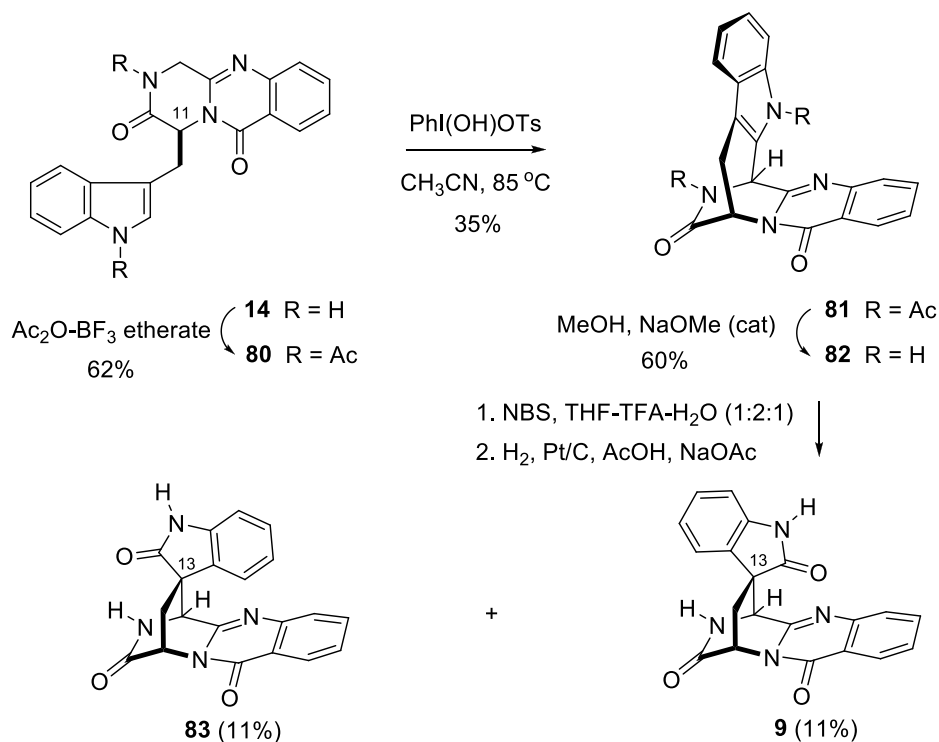
Scheme 13. Enantioselective synthesis of lapatin B 9 .
