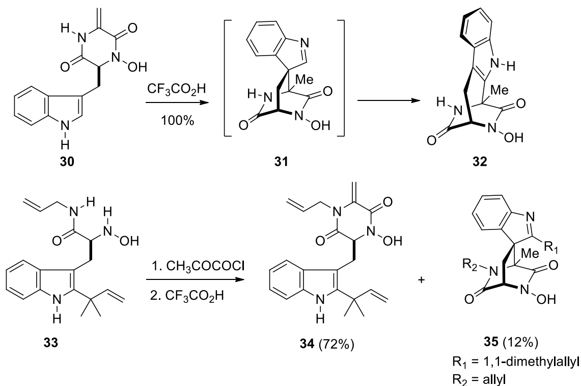
Scheme 2. Ottenheim's studies in the field of diketopiperazine chemistry.
