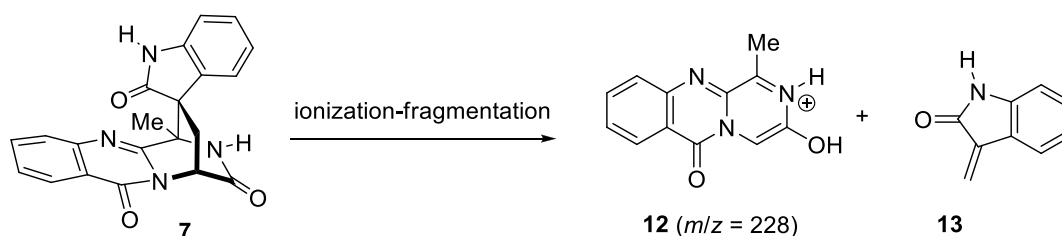
Figure 6. Retro-Diels-Alder fragmentation is typical of spiroquinazoline alkaloids.
