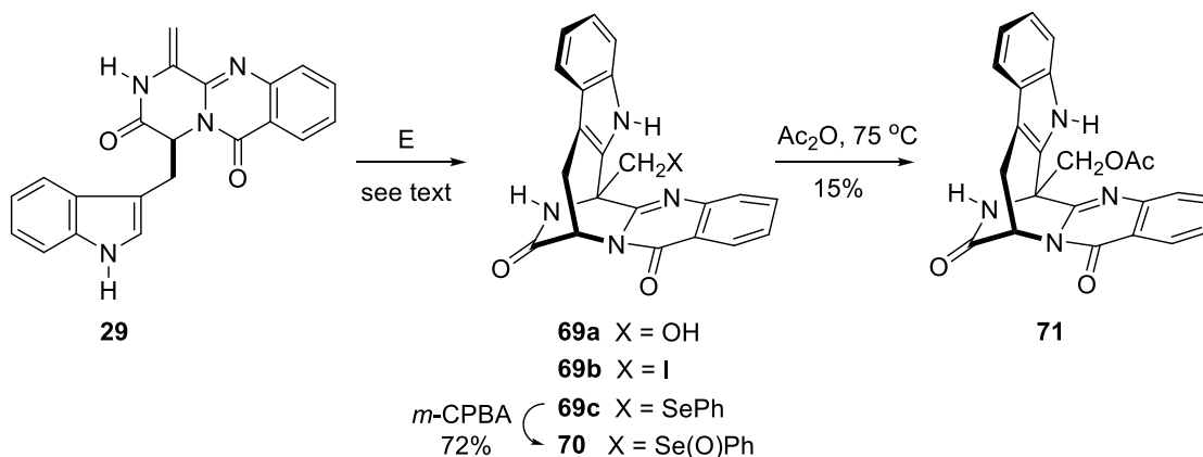
Scheme 10. Unexpected conversion of selenoxide 70 to acetate 71 .
