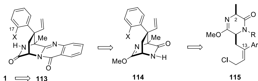
Scheme 20. Chen-Williams approach to synthesis of spiroquinazolines.
