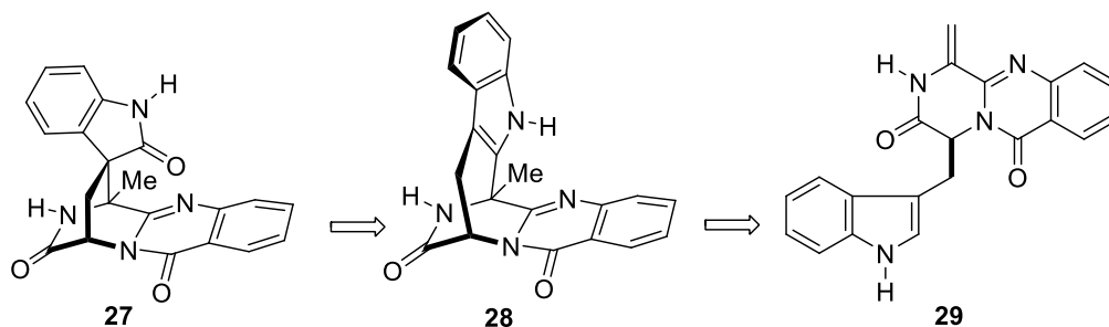
Scheme 1. Plan for synthesis of ent -alantrypinone 27 .
