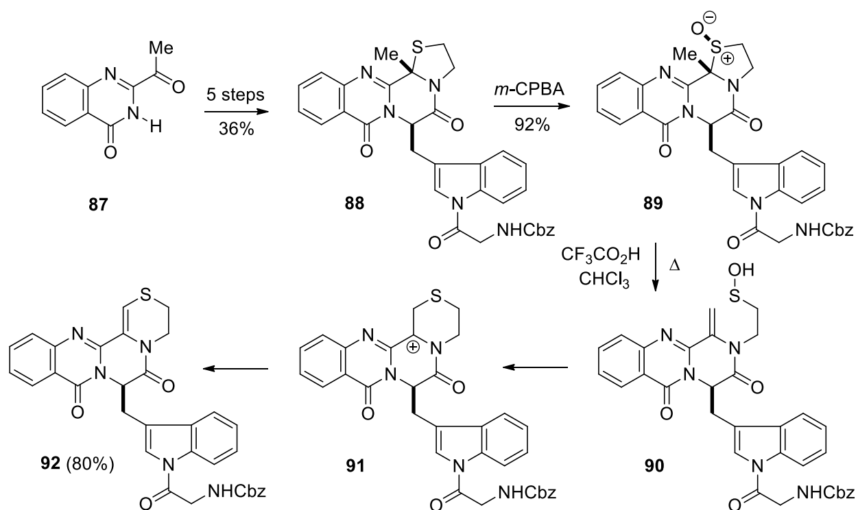
Scheme 15. Failure to capture a possible intermediate cation with an N -acylated indole.
