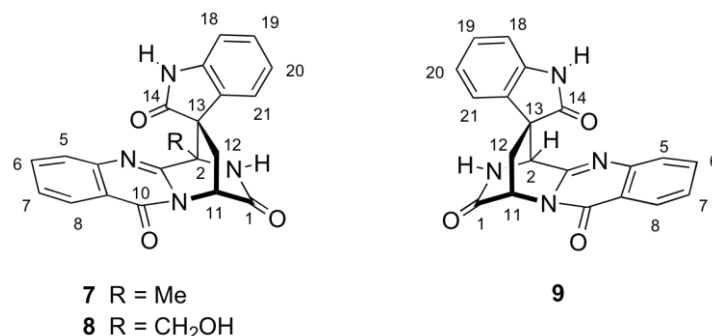
Figure 4. Structures of alantrypinone 7 , serantrypinone 8 and lapatin B 9 .
