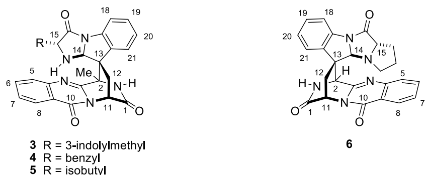
Figure 3. Structures of alanditrypinone 3 , alantryphenone 4 , alantryleunone 5 and quinadoline B 6 .
