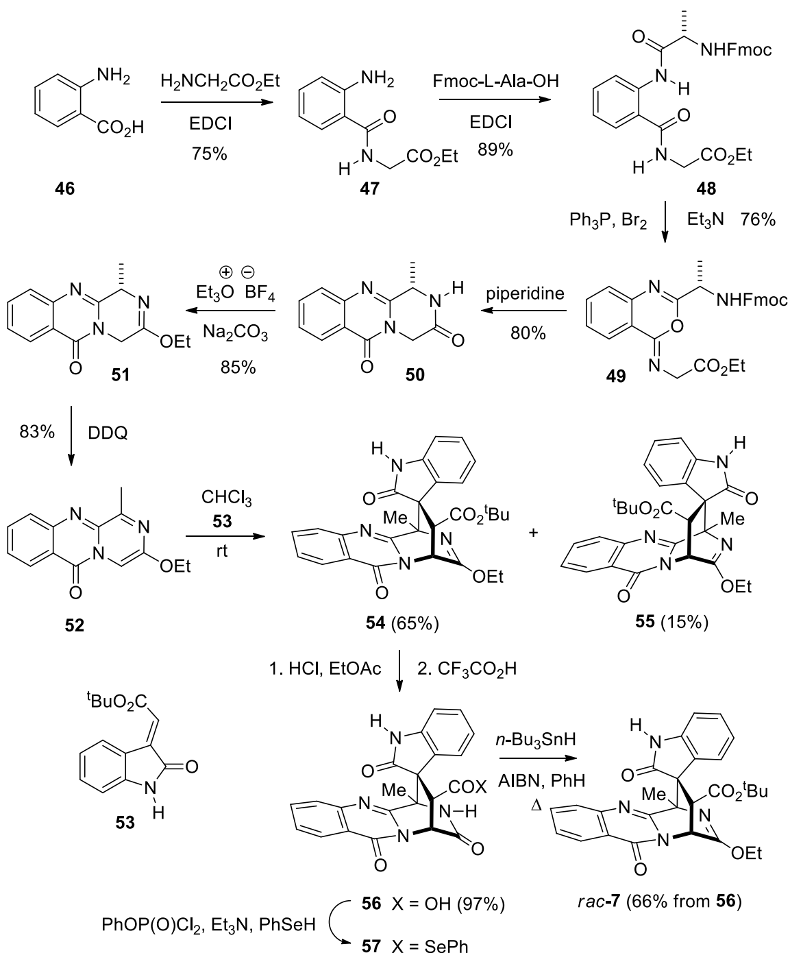
Scheme 5. Kende's first generation synthesis of racemic alantrypinone ( rac -7).
