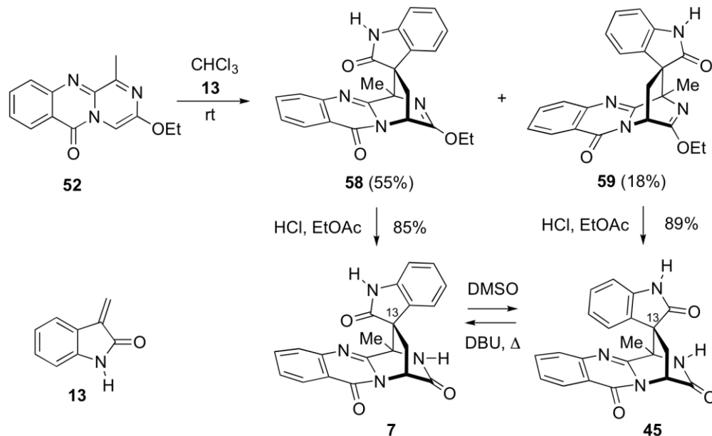
Scheme 6. Kende's second generation synthesis of racemic alantrypinone ( rac - 7 ).
