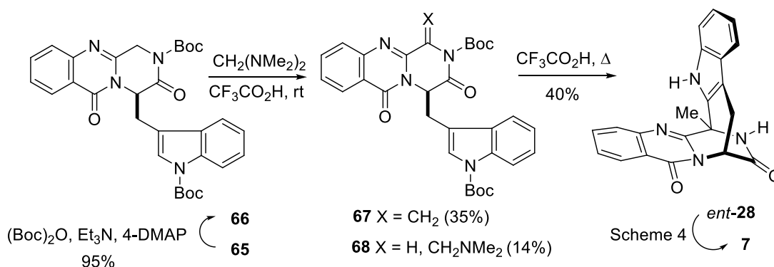
Scheme 9. Completion of Avendaño's formal synthesis of alantrypinone 7 .
