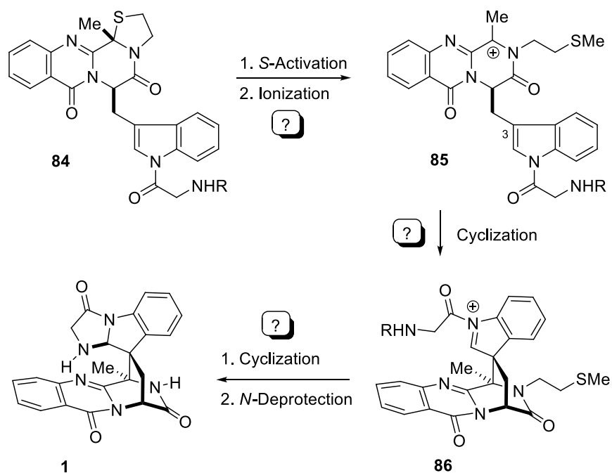
Scheme 14. Plan for conversion of 84 to spiroquinazoline 1 via a cyclization cascade.
