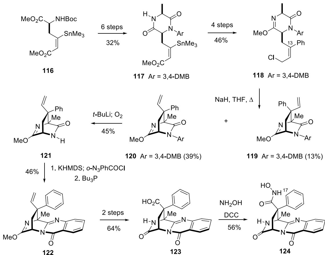
Scheme 21. Synthesis of hydroxamic acid 124 from amino acid 116 .
