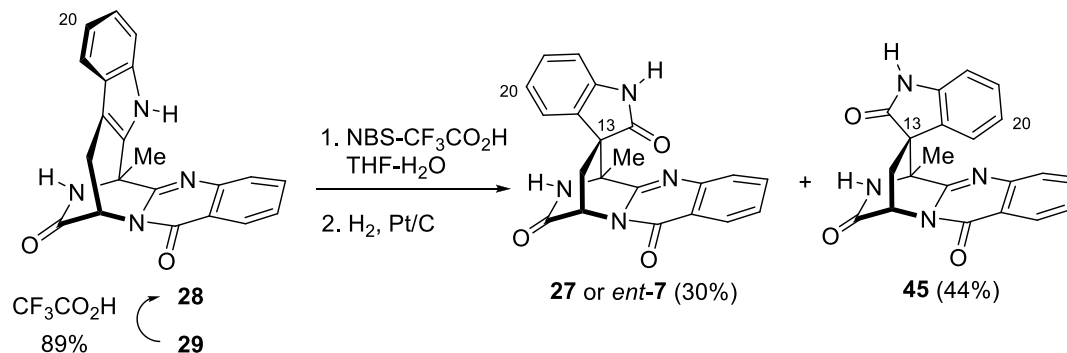
Scheme 4. Synthesis of ent -alantrypinone ( 27 or ent - 7 ) and its C-13 epimer 45 .
