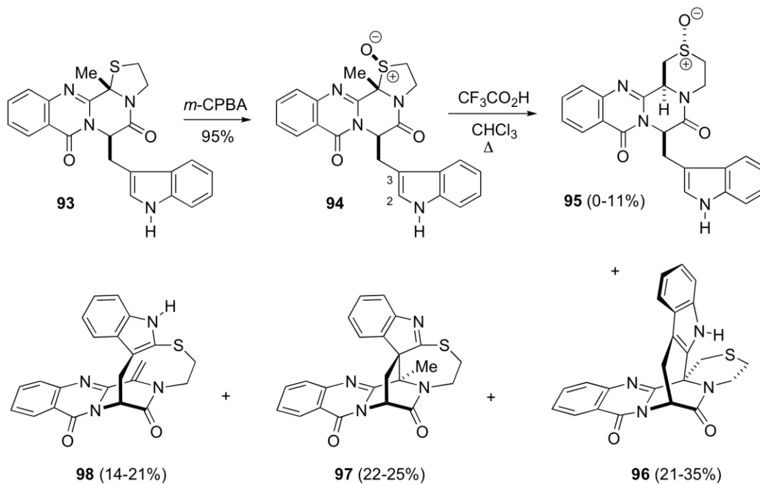
Scheme 16. Acid promoted chemistry of 94 provides structures related to the spiroquinazolines.
