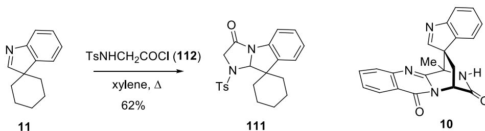
Scheme 19. Conversion of imine 11 to N,N -acetal 111 .
