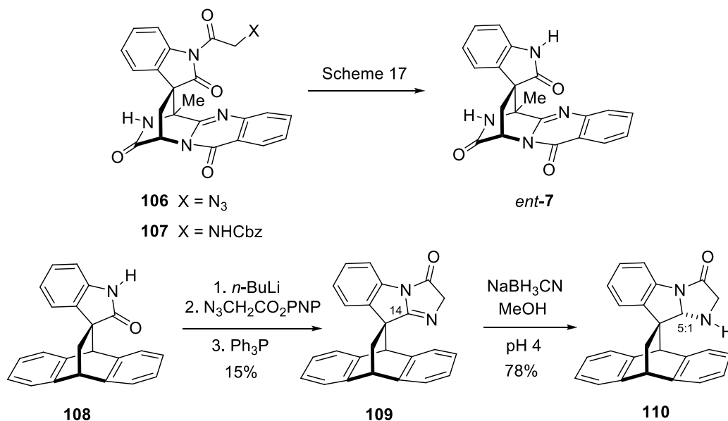
Scheme 18. More model studies for conversion of alantrypinone to spiroquinazoline.
