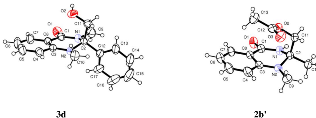
Figure 1. ORTEP 17 views of compounds 3d and 2b' displaying the thermal ellipsoids at 40% probability.
