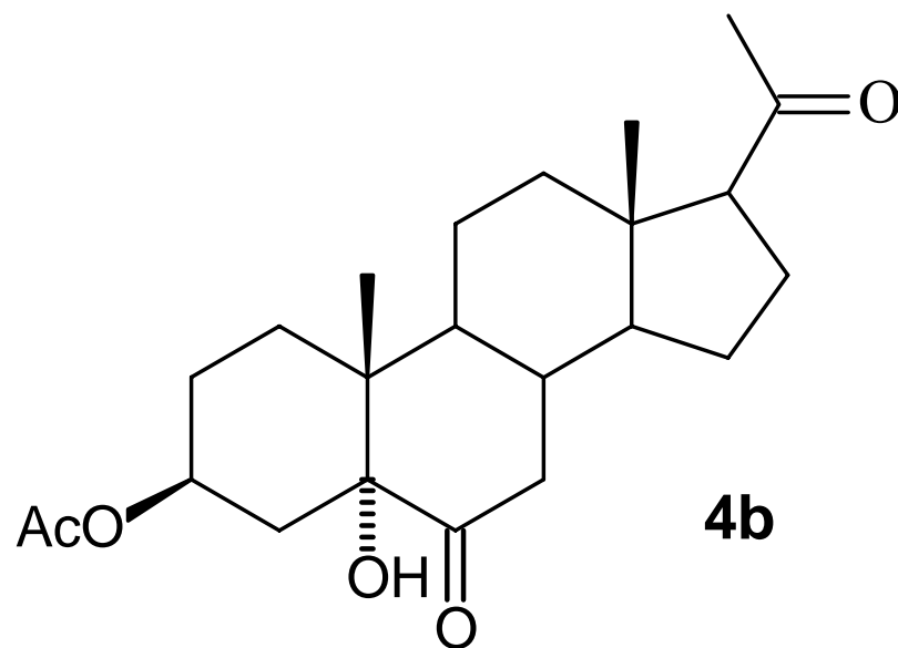
3β-acetoxy-5-hydroxy-5α-pregnan-6,20-dione
