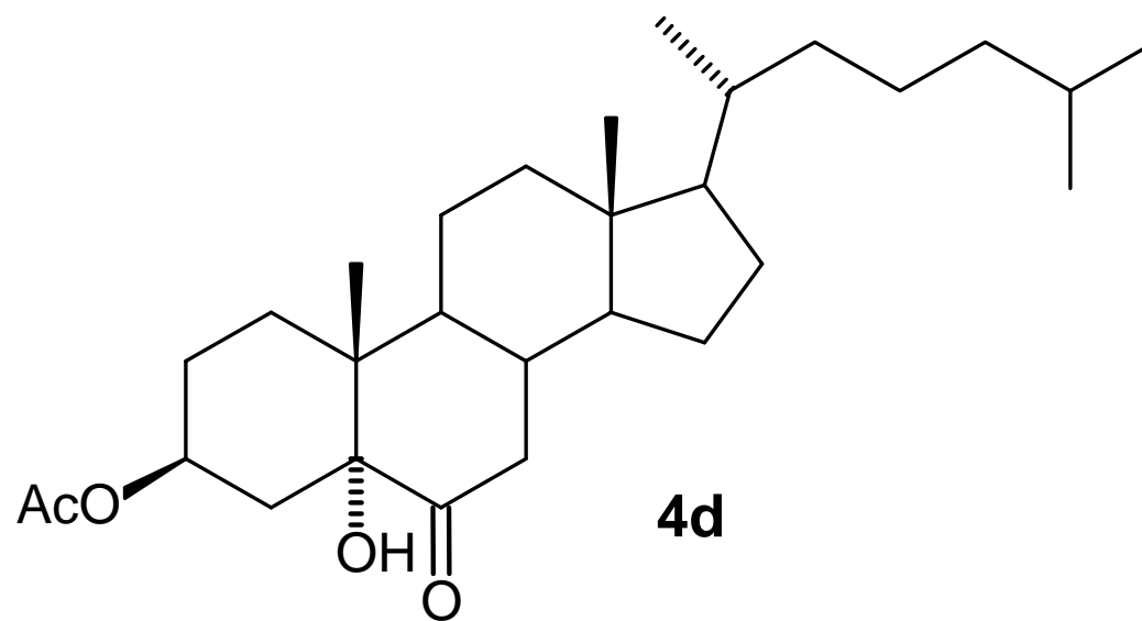
3β-acetoxy-5-hydroxy-5α-cholestan-6-one
