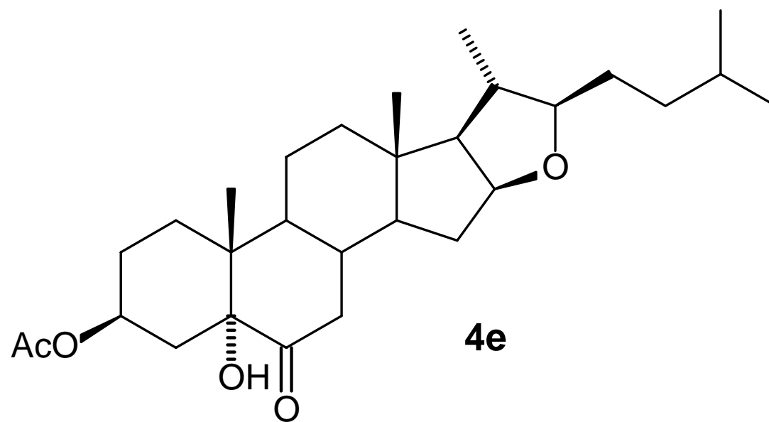
(22 R )-3β-acetoxy-5-hidroxy-5α-furostan-6-one
