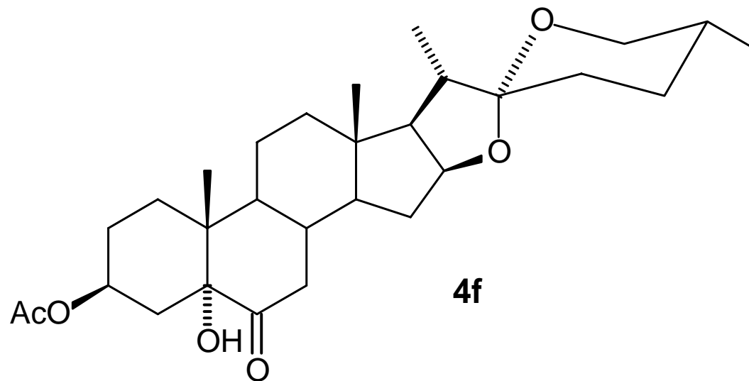
(25 R )-3β-acetoxy-5-hydroxy-5α-spirostan-6-one
