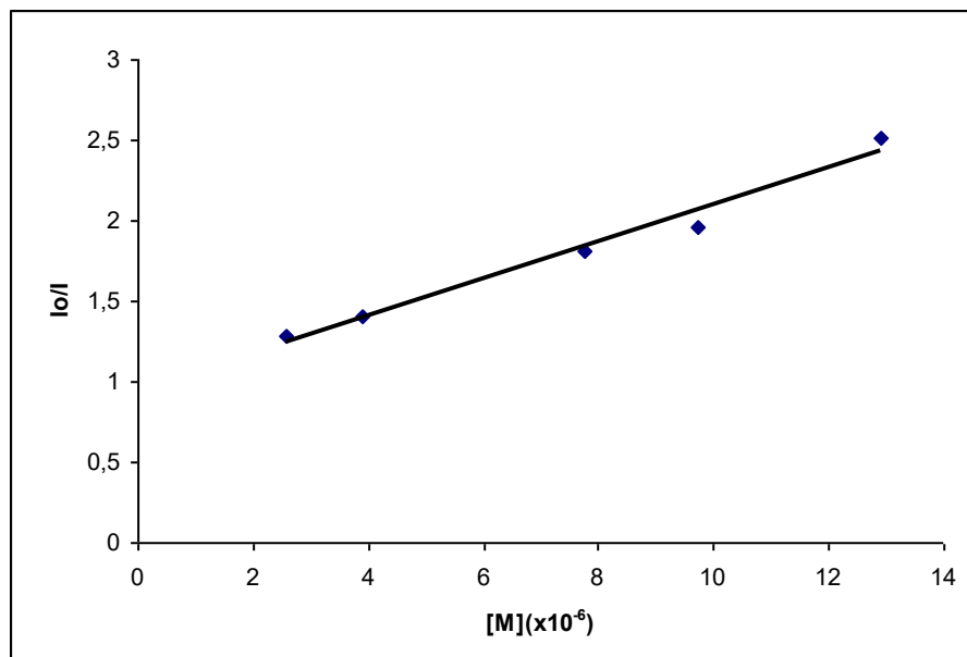
Figure 6. Stern-Volmer plot for the fluorescence quenching of L2 by \text{Pb}^{2+} in MeCN.
