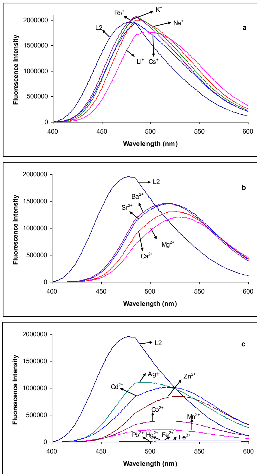
Figure 4. Effect of metal cations on the fluorescence spectra of L2 in MeCN: (a) for alkali metal cations; (b) for alkaline earth metal cations ; (c) for transition metal cations and \text{Pb}^{2+} .
