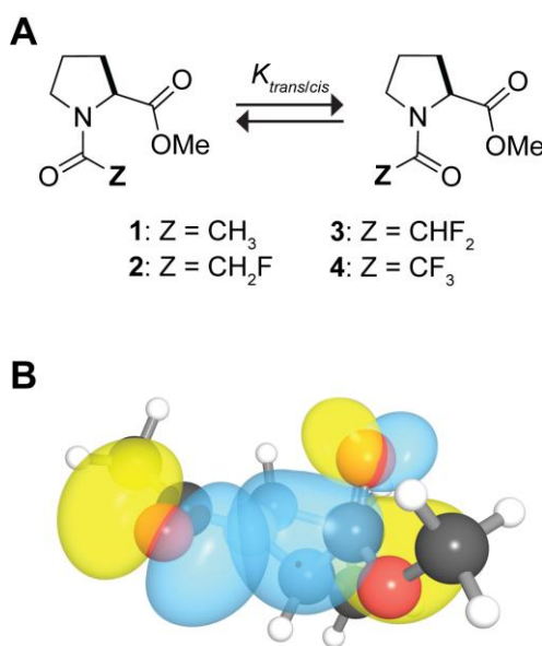
Figure 1. Z-C(O)-Pro-OMe model system: A. Cis – trans equilibrium in Z-C(O)-Pro-OMe.
