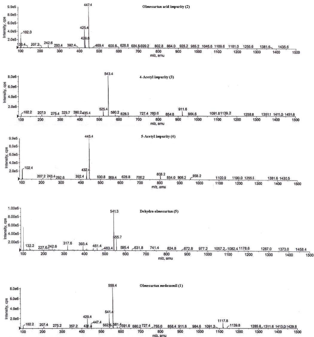
Figure 3. LC-MS Spectrum of olmesartan medoxomil and its related substances.
