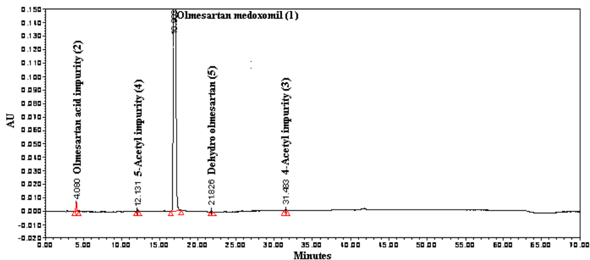
Figure 2. HPLC Chromatogram of olmesartan medoxomil.
