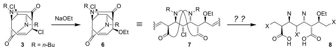
Scheme 2. Unique reactivity of the dichloride and the potential to generate stereochemically rich structures.
