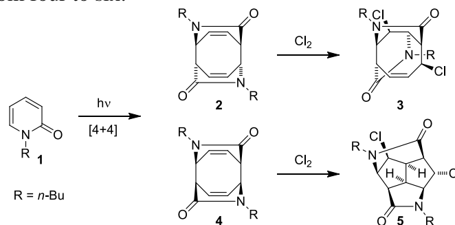
Scheme 1. Photodimerization of 2-pyridone and the major products resulting from chlorination of the trans - and cis - adducts, 2 and 4 , respectively. 5,6
