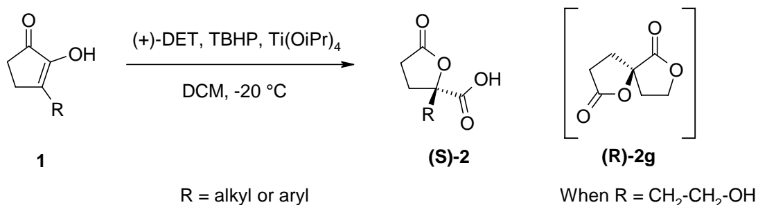
Scheme 1. Asymmetric synthesis of chiral lactone carboxylic acids.
