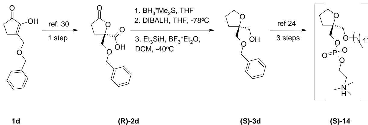
Scheme 4. Formal synthesis of (S)-SRI-62-834 14 .
