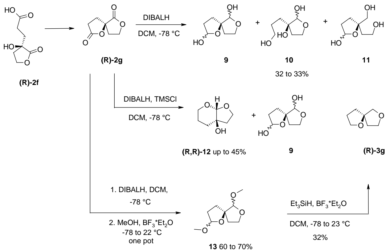
Scheme 5. Synthesis of spirodiether.
