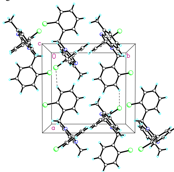
Figure 4. Unit cell of 3r showing all the weak interactions.
