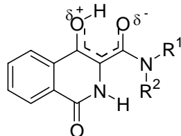
Figure 3. RAHB effect in N -lactam unsubstituted isoquinolinones.
