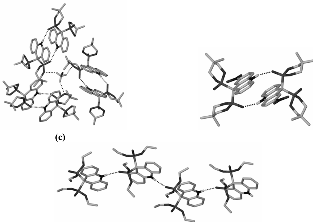
Figure 2. Drawings showing hydrogen-bonding interactions in (a) 11 .CH 3 CN, (b) 14 .OC 4 H 8 , and (c) 17 . Hydrogen-bonding interactions: Compound 11 .CH 3 CN (Å, °): N(1)-H(1A)...O(3') 0.77(4), 2.18(4), 2.952(7), 176(4); C(25)-H(25A)...O(2) 1.07(7), 2.41(8), 3.361(8), 147(6). Symm. Equiv.: 5/3-x, 4/3-y, 1/3-z. Compound 14 .OC 4 H 8 N(1)-H(1A)...O(6') 0.86, 1.99, 2.820(6), 162.5. Symm. Equiv.: 2-x, 1-y, -z. Compound 17 N-H(1A)...O(4') 0.78(5), 2.18(5), 2.910(6), 155(5). Symm. Equiv.: 2-x, 0.5+y, -z.
