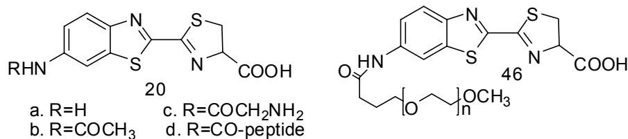
Figure 8. Structure of 6'-aminoluciferin ( 20a ), amides 20b,c,d and PEGylated aminoluciferin 46 .
