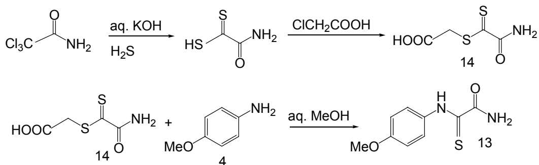
Scheme 3. In situ preparation of carbamoylthiocarbonylthioacetic acid 14 and preparation of compound 13 . 12,13
