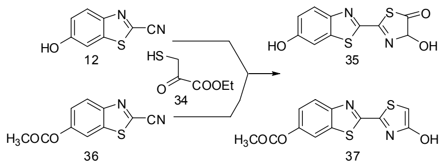
Scheme 11. Synthesis of oxyluciferin derivatives 35 and 37 . 52,53
