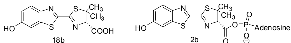
Figure 5. Structure of compounds 18b and 2b .
