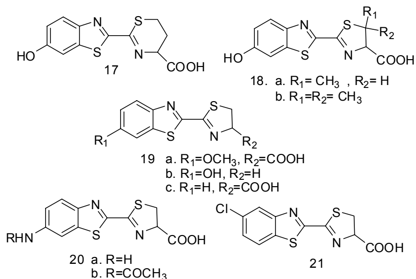
Figure 2. Structure of compounds 17 , 18 , 19 , 20 , and 21 .
