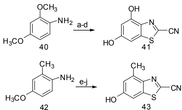
Scheme 12. Synthesis of nitriles 41 and 43 , intermediates of 4'-substituted D-luciferin analogues 39a,b . 55,56 Reagents and conditions: (a) carbamoylthiocarbonylthionoacetic acid, aq. EtOH, r.t., 48.6%; (b) K 3 [Fe(CN) 6 ], NaOH 1M, 10 °C, 30 min, 77%; (c) POCl 3 in Py, r.t., 2 h, 90%; (d) PyHCl, 170-180°C, 3 h, 56%; (e) ethyl oxalate, 180 °C, 5 min, 65%; (f) P 2 S 5 , xylene, reflux, 2h; NaOH, r.t.; (g) K 3 [Fe(CN) 6 ], NaOH 1M, <10 °C, 66% from oxamate; (h) SOCl 2 , reflux, 2h, 40%, (i) POCl 3 , reflux, 15 min, 67%; (j) PyHCl, 220 °C, 1h, 7%.
