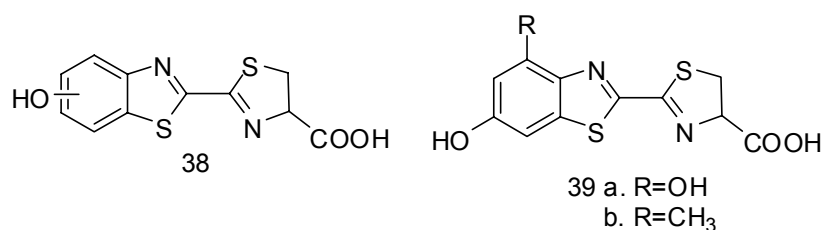
Figure 6. Structure of phenolic regioisomers of D-luciferin (compounds 38 ) and of 4'-substituted- D-luciferin analogues 39a,b .
