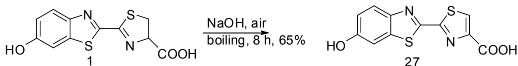
Scheme 7. Synthesis of dehydroluciferin 27 from D-luciferin 1 . 9
