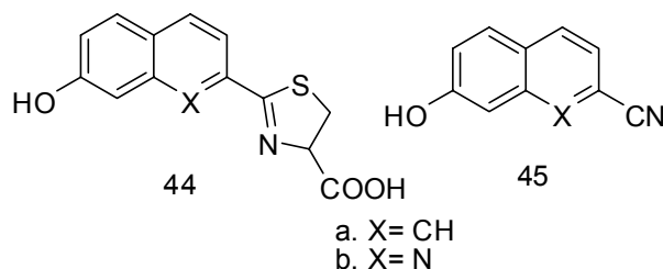
Figure 7. Structure of naphthalene and quinoline derivatives 44a,b and structure of nitriles 45a,b .
