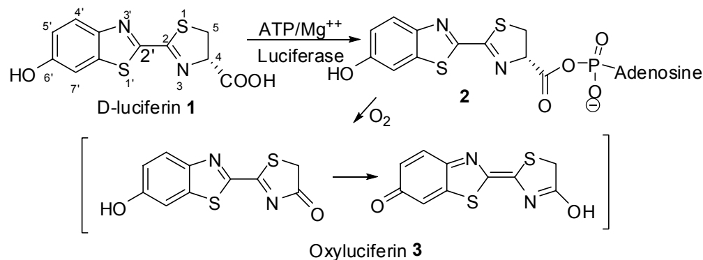
Figure 1. Luciferase-catalyzed transformation of D-luciferin ( 1 ) into oxyluciferin ( 3 ).
