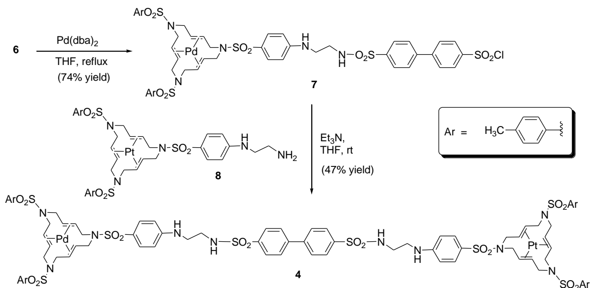
Scheme 3. Synthesis of Pd 0 -Pt 0 heterobimetallic complex 4 .
