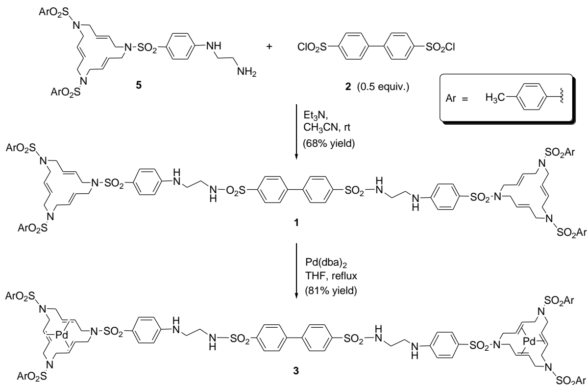
Scheme 1. Synthesis of 15-membered triolefinic bismacrocylic ligand 1 and its bispalladium(0) complex 3 .
