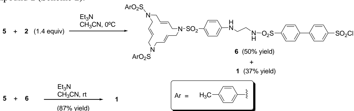
Scheme 2. Stepwise synthesis of 15-membered triolefinic bismacrocylic ligand 1 .
