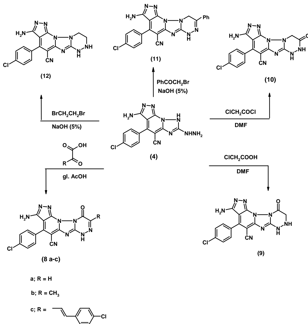
Scheme 2. Synthetic pathway for the preparation of compounds 8-12.
