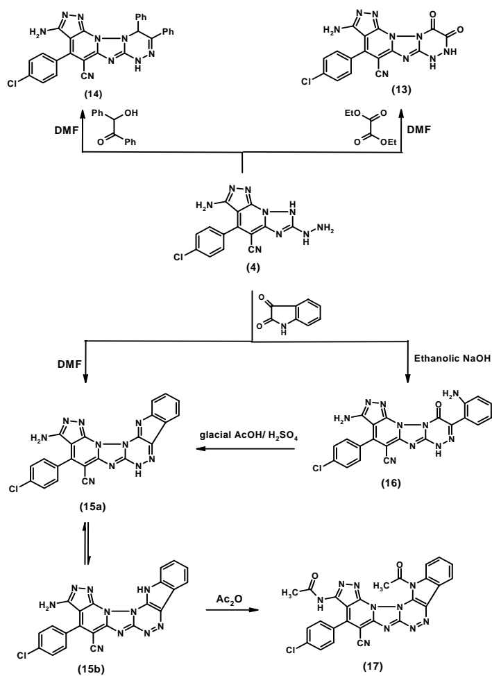
Scheme 3. Synthetic pathway for the preparation of compounds 13-17.
