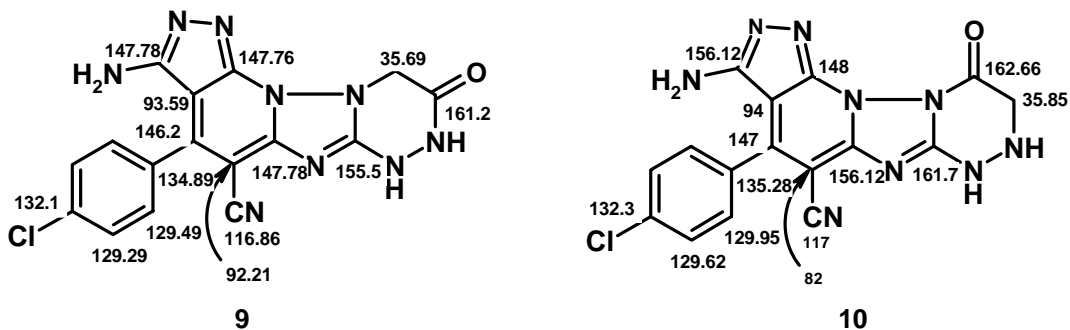
Figure 1. 13 C NMR of compounds 9 and 10.
