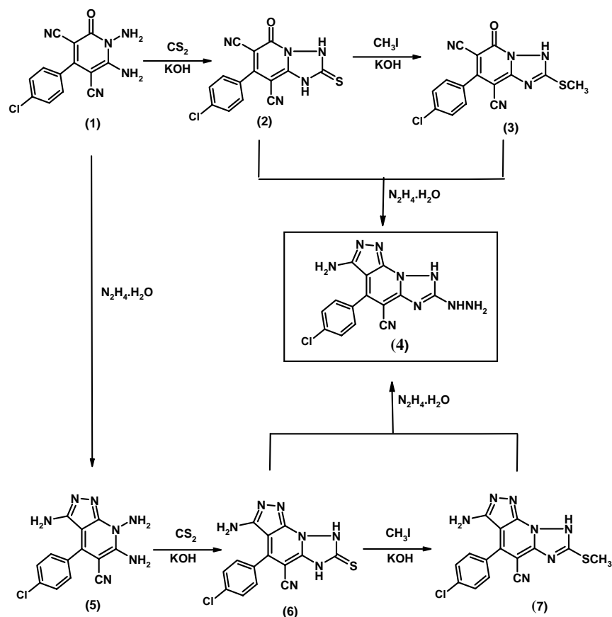
Scheme 1. Synthetic pathway for the preparation of target compound 4 .
