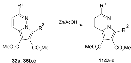
114a: R1=R2=Me; 114b: R1=Ph, R2=H; 114c: R1=4-MeC6H4 R2=H
