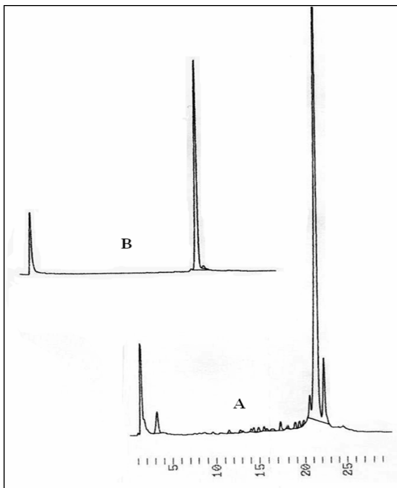
Figure 1. A - IE HPLC trace of reaction mixture, resulting from cleavage/deprotection of CPG bound protected 5'-ATACCGATTAAGCGAAGTTT X TTA-3'. The major peak, eluting at 21.5 min corresponds to the deprotected 20mer oligonucleotide 5'-ATACCGATTAAGCGAAGTTT-3', N-OH. The minor peak, eluting at 22.5 min corresponds to 24mer ATACCGATTAAGCGAAGTTTYTTA-3', f . B - standard 20mer oligonucleotide 5'-ATACCGATTAAGCGAAGTTT-3', N-OH, retention time ( \tau_R ) 21.5 min.
