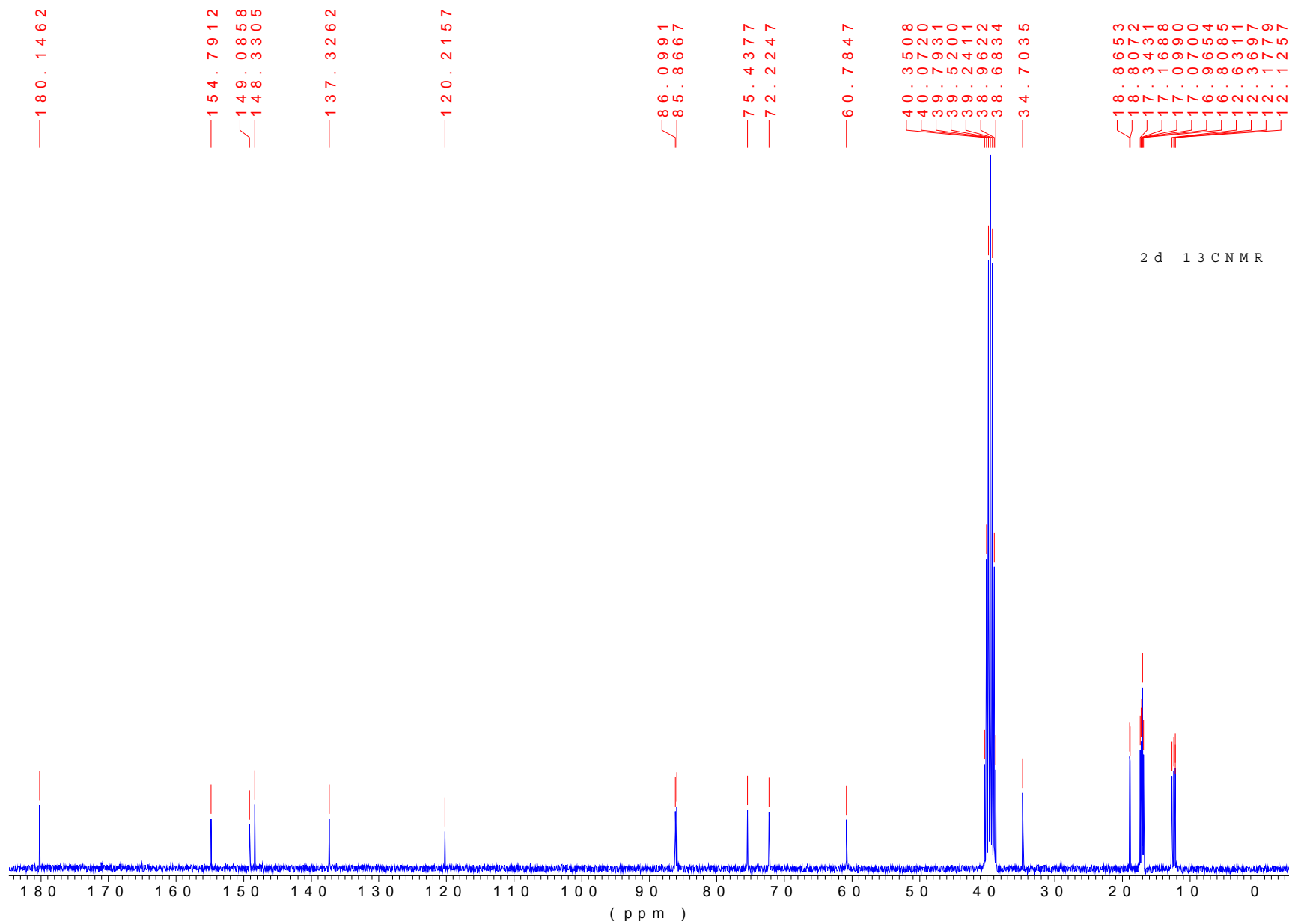
13 C NMR spectrum (75 MHz) of N 2 -Isobutyryl-2',3'-O-(1,1,3,3-Tetraisopropylidisiloxane-1,3-diyl)guanosine ( 2d ) in DMSO-d 6 at 300 K.
