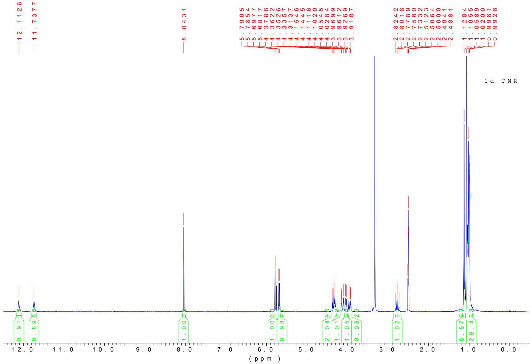
^1\text{H} NMR spectrum (300 MHz) of \text{N}^2 -Isobutyryl-3',5'-O-(1,1,3,3-tetraisopropyldisiloxane-1,3-diyl)guanosine ( 1d ) in \text{DMSO-d}_6 at 300 K.
