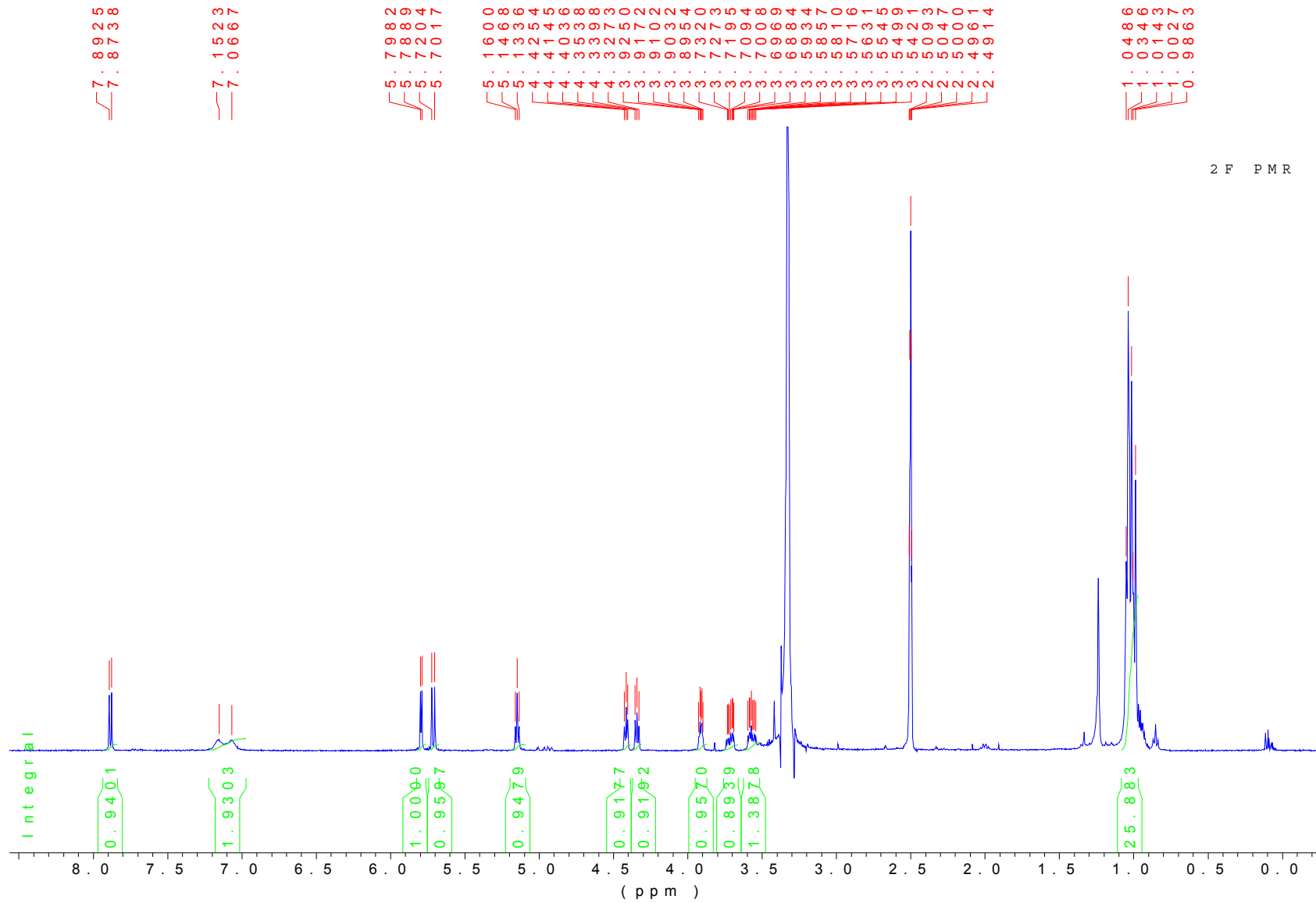
^1\text{H} NMR spectrum (400 MHz) of 2',3'-O-(1,1,3,3-Tetraisopropylidisiloxane-1,3-diyl)cytidine ( 2f ) in DMSO- d_6 at 300 K.
