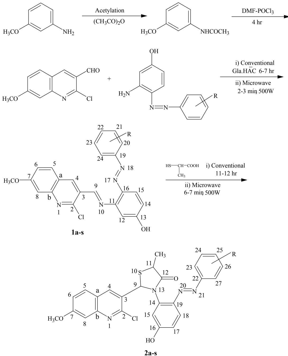
Scheme 1. R= -H, 2-OCH 3 , 3-OCH 3 , 4-OCH 3 , 2-Br, 3-Br, 4-Br, 2-Cl, 3-Cl, 4-Cl, 2-NO 2 , 3-NO 2 , 4-NO 2 , 2-CH 3 , 3-CH 3 , 4-CH 3 , 2-F, 3-F, 4-F
