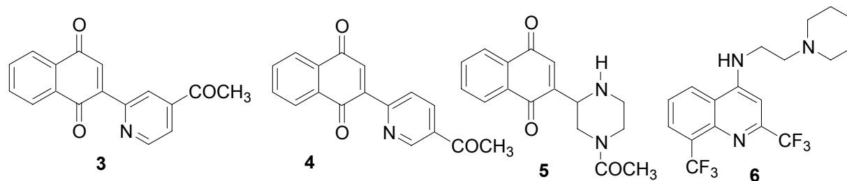
Figure 2. Naphthoquinone and aminoquinoline derivatives.
