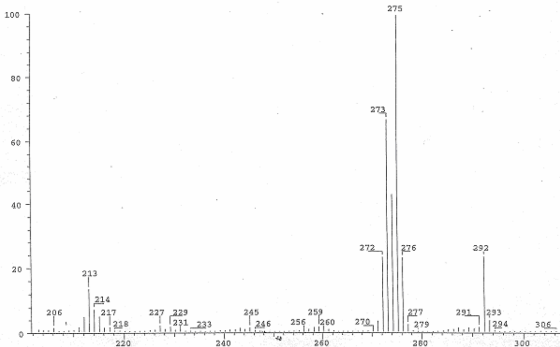
Figure 8. FAB MS spectra of the N-CD 3 -dextromethorphan base.
