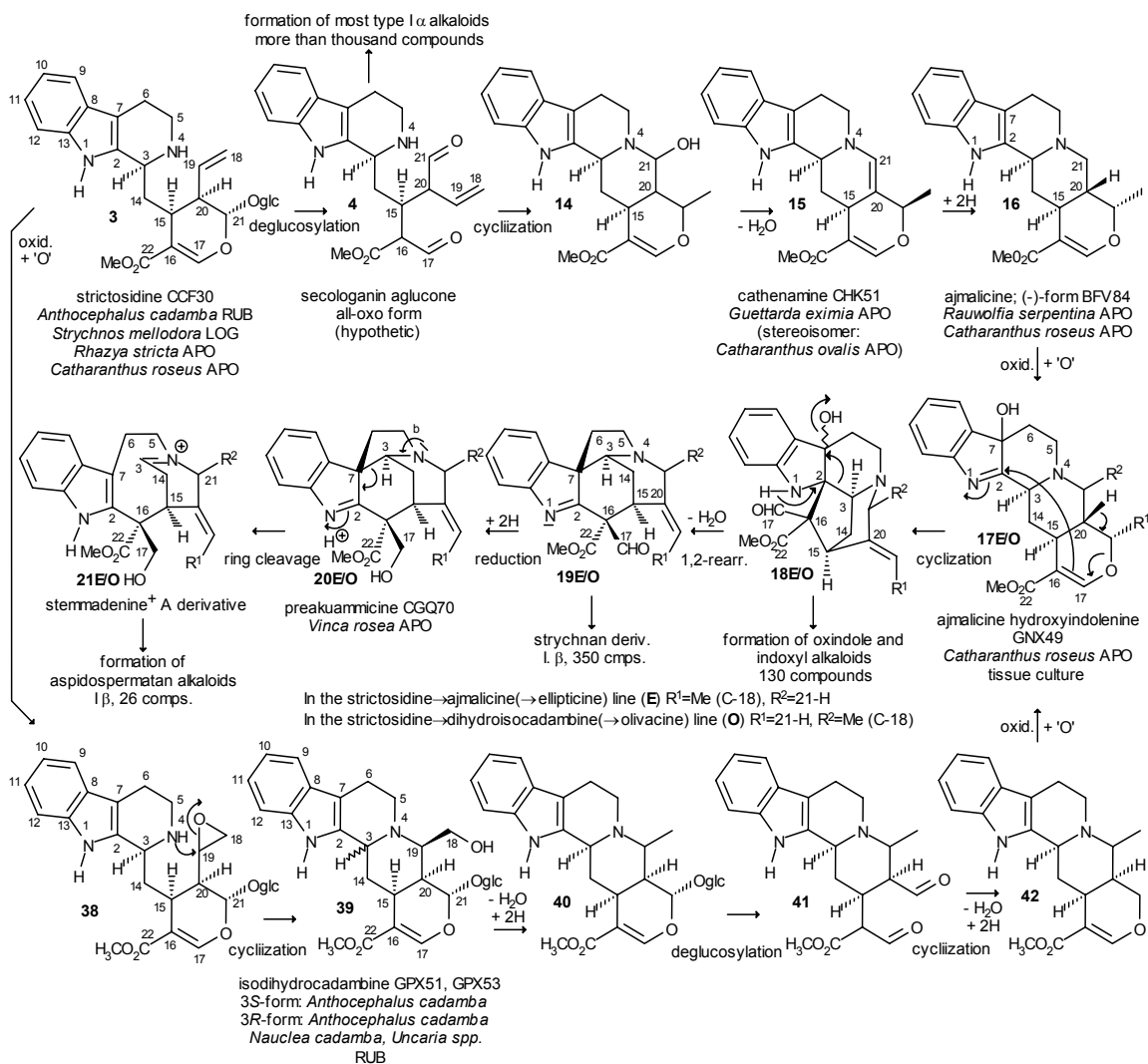
Scheme 4. Generation of ellipticine and olivacine. Part 1.
