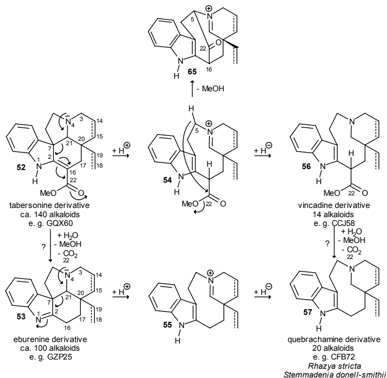
Scheme 9. Long-range interaction in the plumeran skeleton.
