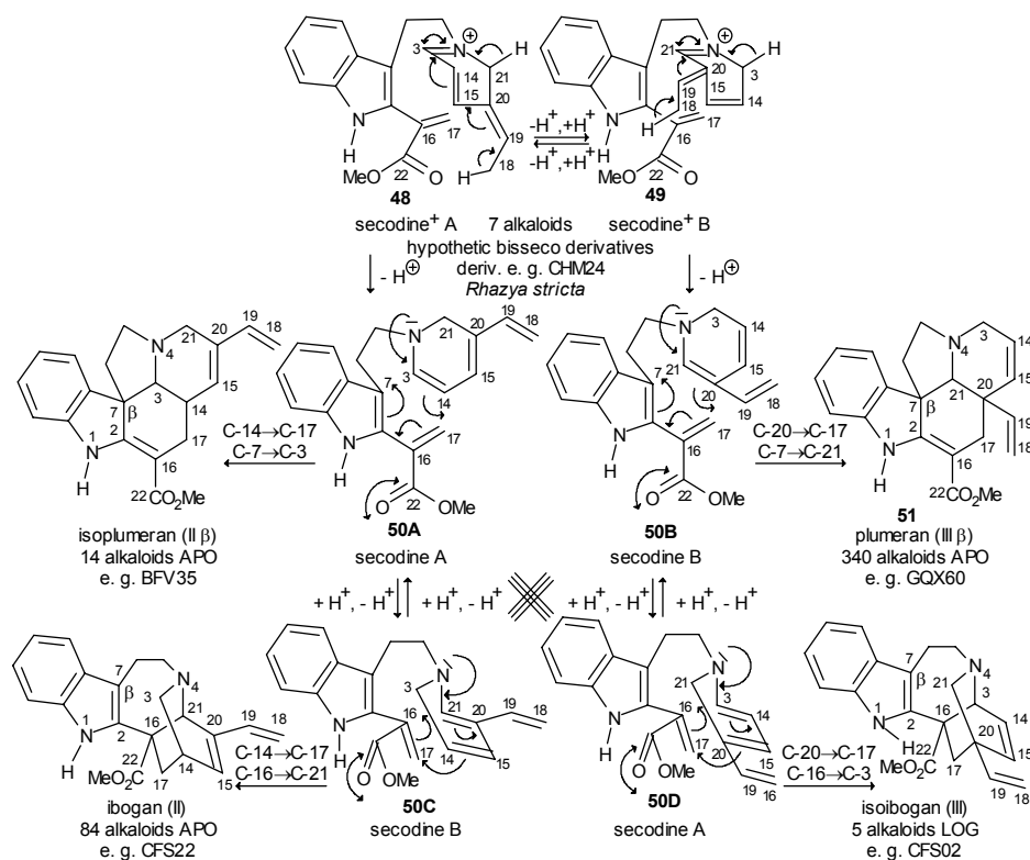
Scheme 8. Formation and transformation of the secodine structure.
