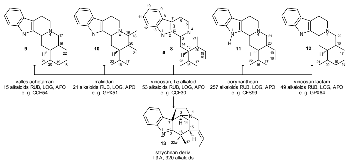
Scheme 3. Primary cyclizations in type I \alpha indole alkaloids.
