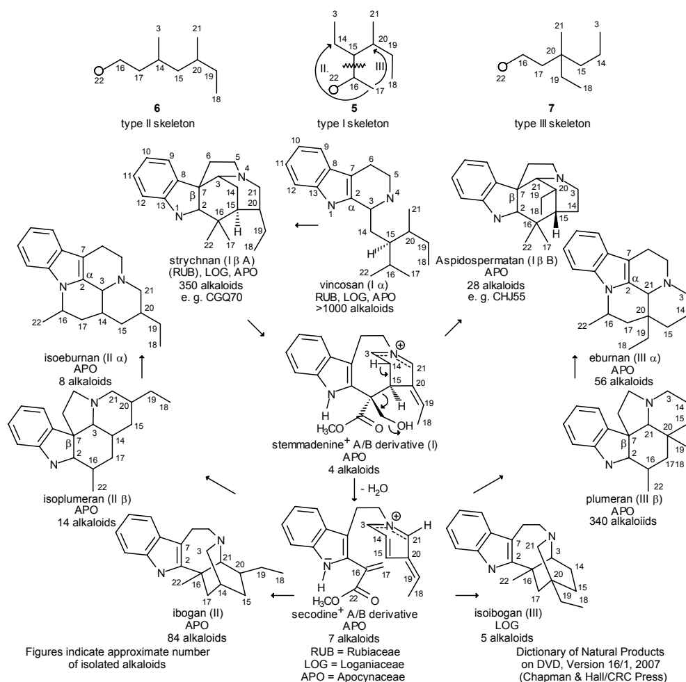
Scheme 2. Biogenetic-type system of indole alkaloids derived from secologanin.
