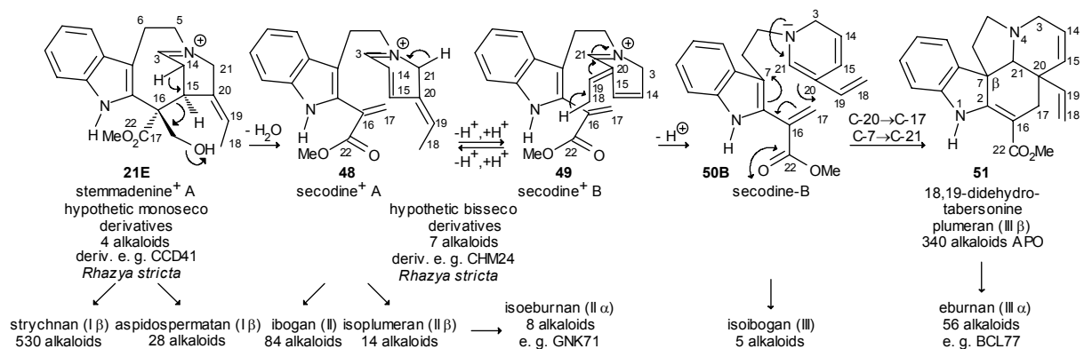
Scheme 7. Generation of rhazinilam and rhazinal. Part 1.
