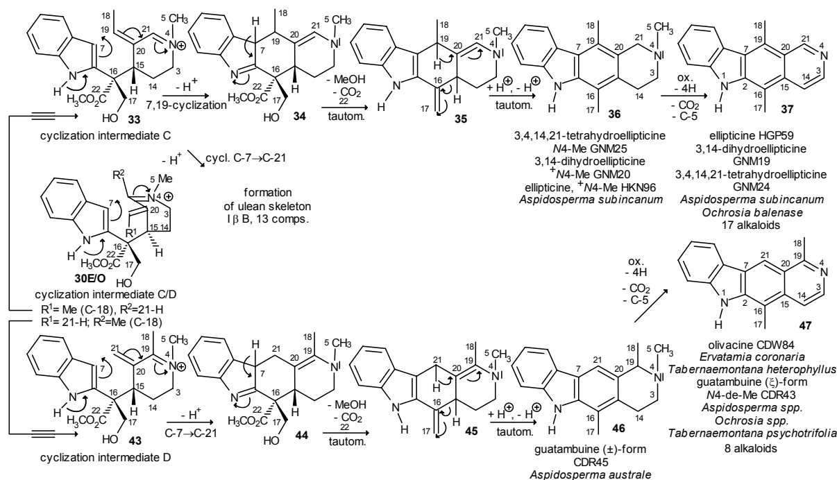
Scheme 6. Generation of ellipticine and olivacine. Part 3.
