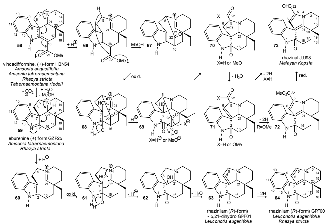
Scheme 10. Generation of rhazinilam and rhazinal. Part 2.
