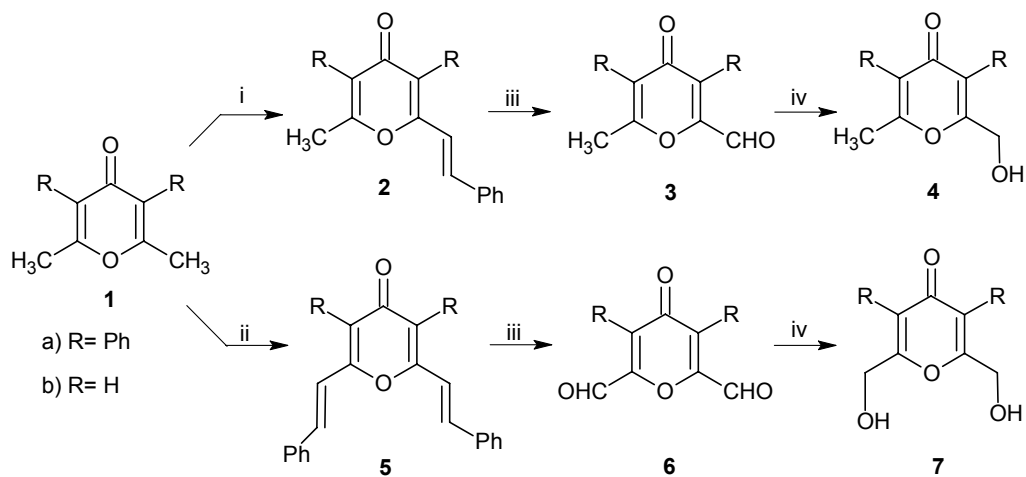
Scheme 1. (i) PhCHO, NaOEt, (ii) 2PhCHO, 2NaOEt, (iii) OsO 4 , KIO 4 , (iv) NaBH 4
