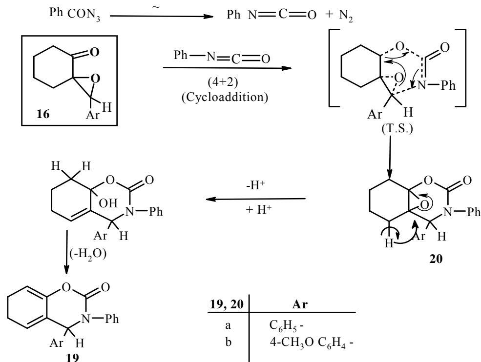
Scheme 8. HHSS based on (4+2) cycloaddition reaction.
