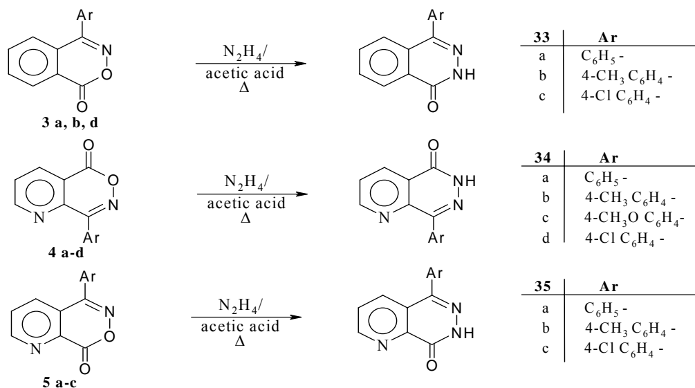
Scheme 13. HHSS based on ANRORC ring transformation.
