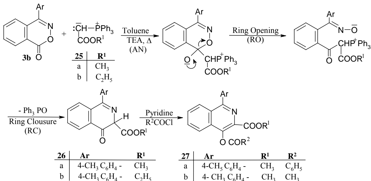
Scheme 11. HHSS based on ANRORC-ring transformation.
