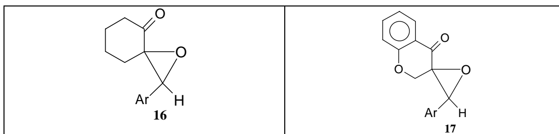
Figure 2. Spirooxiranes
