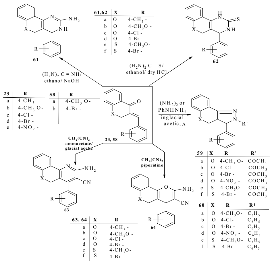
Scheme 19. HHSS based on cyclocondensation.
