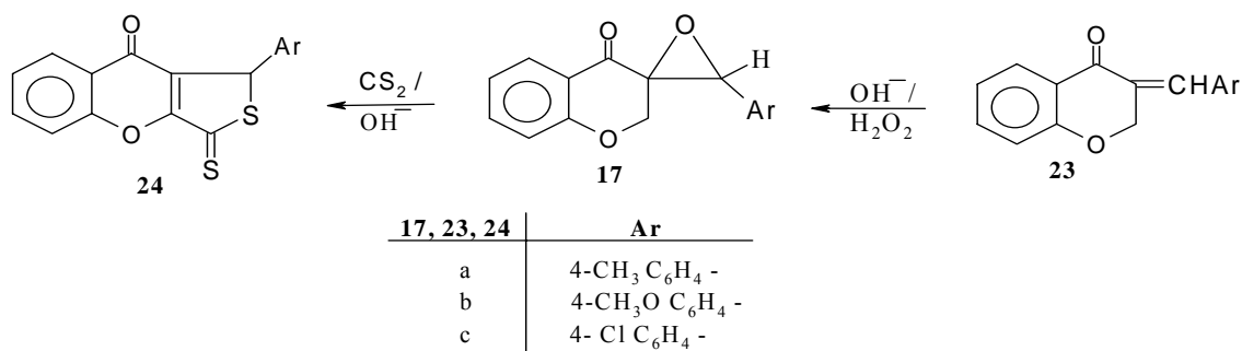
Scheme 10. HHSS based on cycloaddition reaction.
