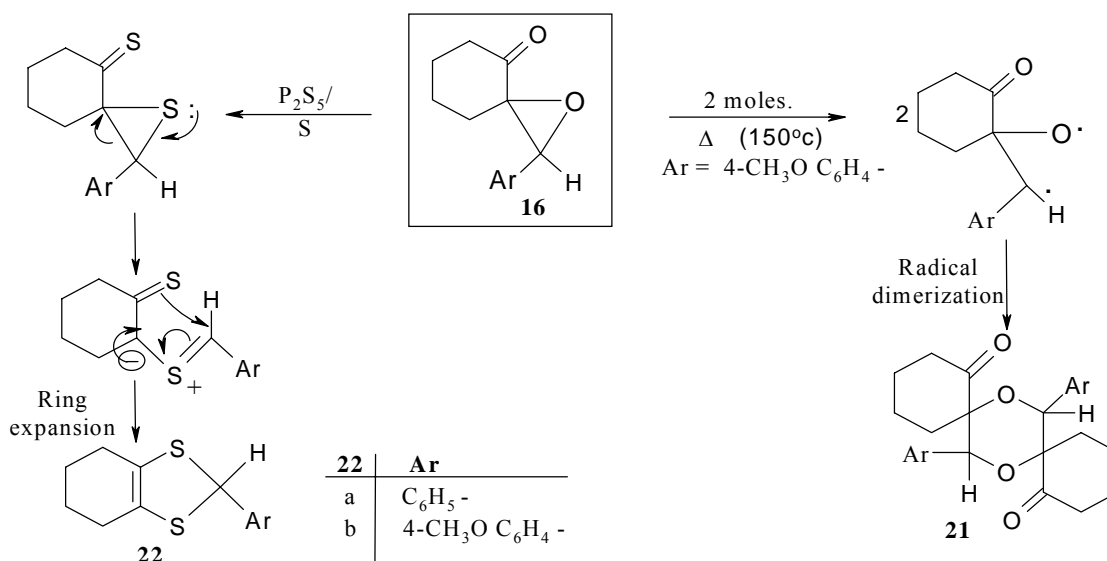
Scheme 9. HHSS based on Ring expansion and radical dimerization reactions.
