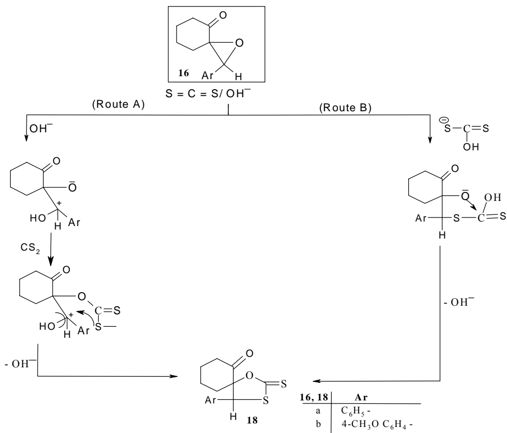
Scheme 7. HHSS based on cycloaddition reaction.
