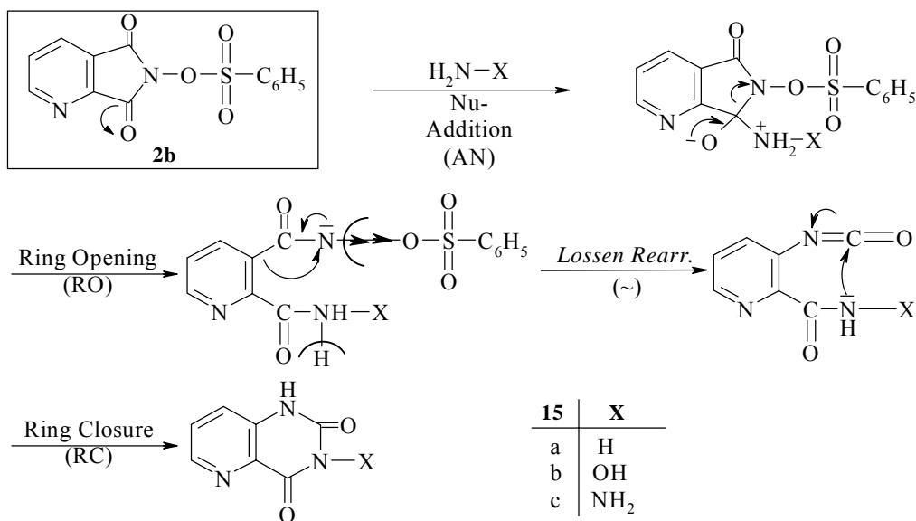
Scheme 6. ANRO ~ RC type ring transformation.
