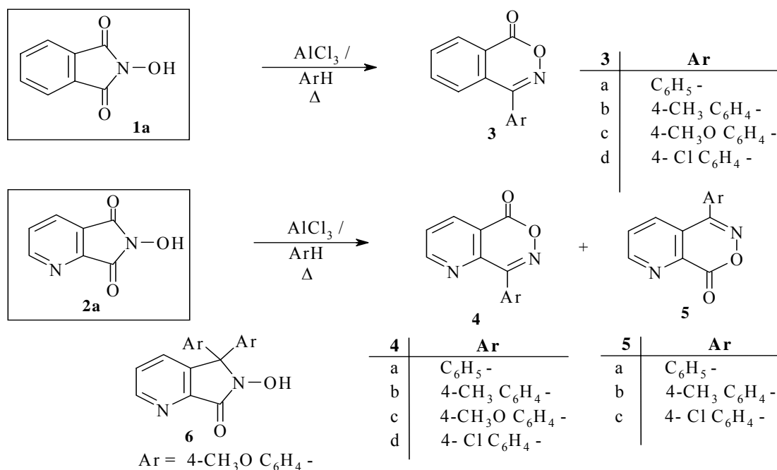
Scheme 1. HHSS based on molecular rearrangements.
