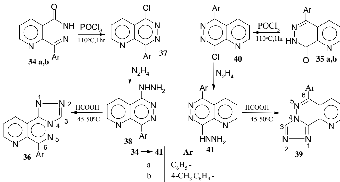
Scheme 14. Three-step synthesis.
