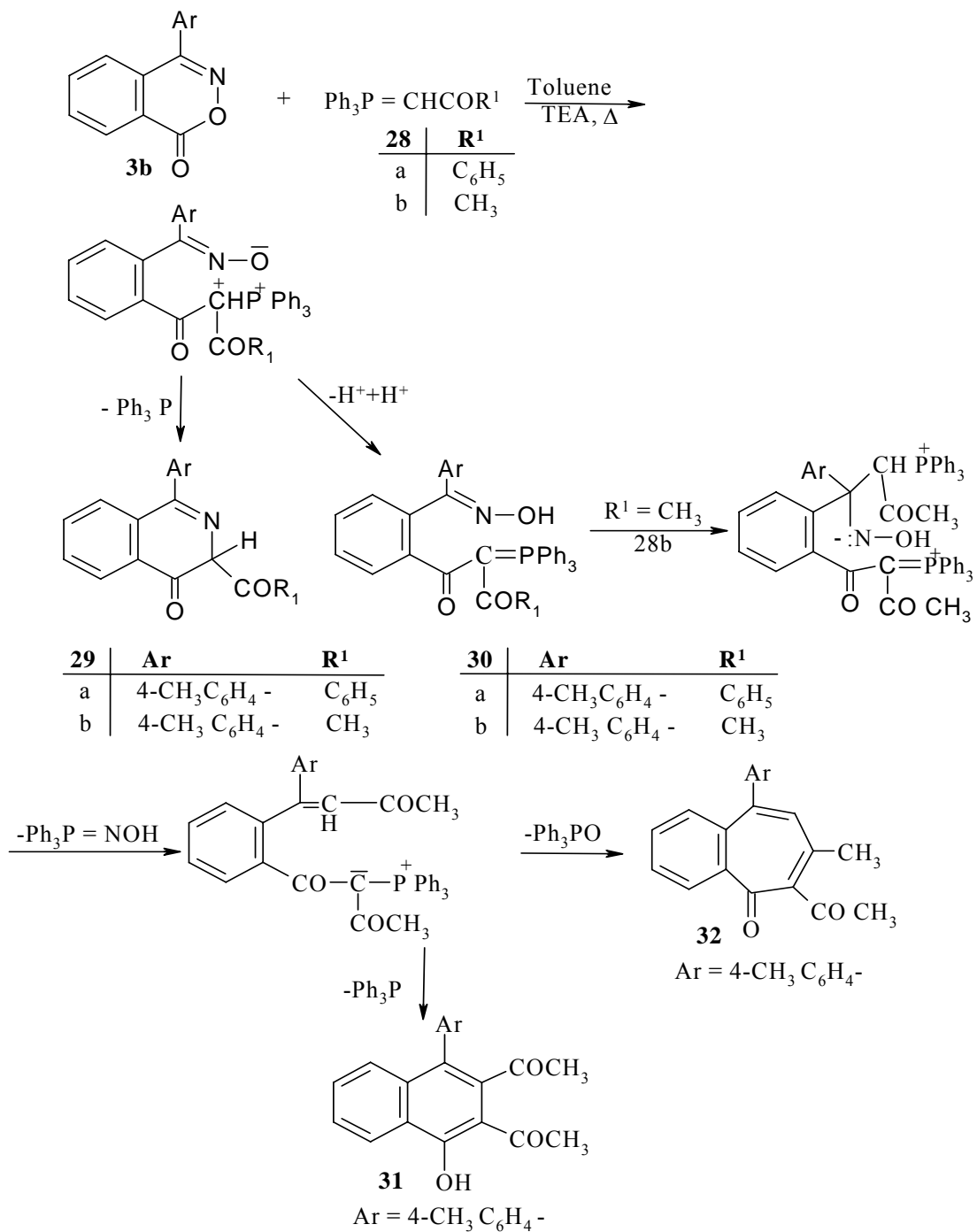
Scheme 12
