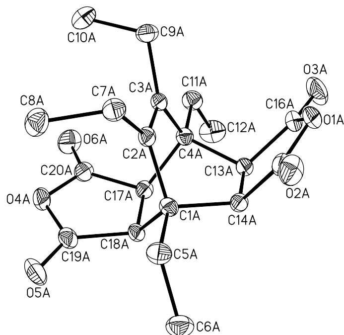
Figure 4. Molecular structure and numbering scheme of 3 . The ellipsoids represent a probability of 40%, the hydrogen atoms are omitted for clarity reasons. Only molecule A is shown. Selected bond lengths (Å): C1A-C2A 1.538(4), C2A-C3A 1.349(4), C3A-C4A 1.535(4), C1A-C14A 1.555(4), C13A-C14A 1.528(4), C4A-C13A 1.567(4), C1A-C18A 1.562(4), C17A-C18A 1.526(4), C4A-C17A 1.555(4).
