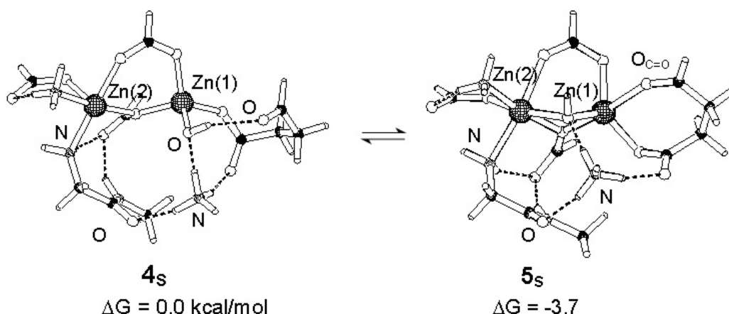
Scheme 5. Stabilization of the docking intermediate 4_S through the generation of a \mu -OH bridge (species 5_S ). Calculated at the B3LYP/aug-cc-pVTZ//B3LYP/lanl2dz level of theory.
