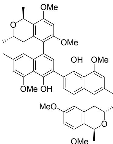
Figure 1. Structure of a synthetic analog of a korupensamine
