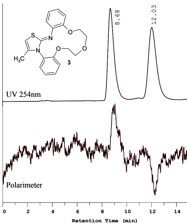
Figure 2. Chromatogram of macrocycle 3 on Chiralcel OD-H column at 25°C (Eluent 80:20 Hexane / 2-PrOH).
