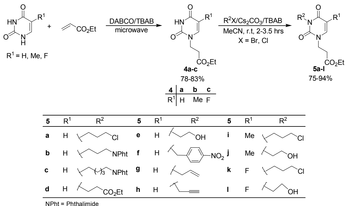
Scheme 1. Synthesis of N 1, N 3-dialkylated pyrimidines.
