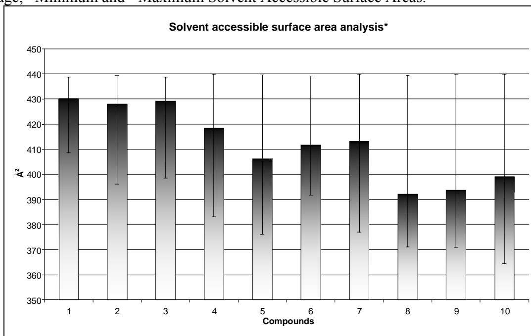
Figure 1. Fluorenone ASASA results for compounds 1-10. *Bar plots refer to the averaged solvent accessible surface area in Å 2 for the fluorenone moiety. Error bars regard the maximum and minimum ASASA values in the conformational ensemble generated in the Monte Carlo search.
