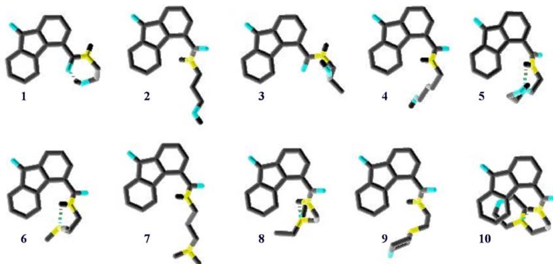
Figure 2. Energy global minimum conformers of compounds 1-10 (polytube models) obtained in the Monte Carlo conformational search. Hydrogen bonds are represented with the dashed lines.
