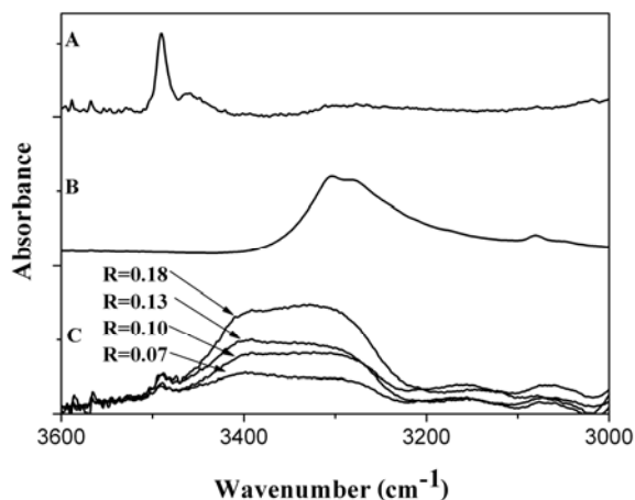
Figure 9. Comparison between FT-IR spectra of MLT/CCl 4 (A), pure MLT (B) and MLT/AOT/CCl 4 system at various R values (C).
