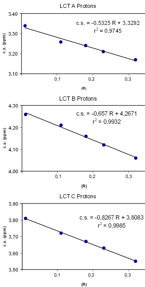
Figure 3. Chemical shift (c.s.) of LCT A, B, C protons as function of R.
