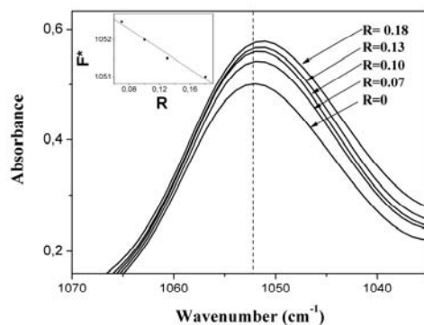
Figure 10. SO 3 - symmetric stretching bands of the MLT/AOT/CCl 4 system at various R values. In the inset is reported the frequency at the band maximum (F*) as a function of R.
