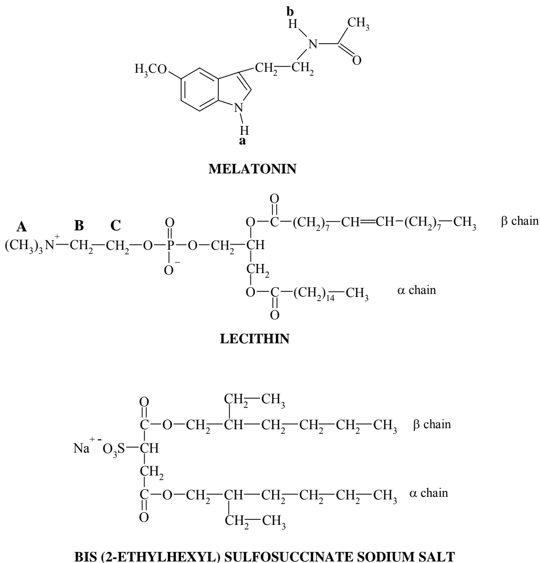
Figure 1. Molecular structures of MLT, LCT and AOT.
