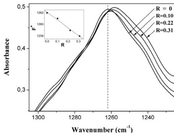
Figure 6. \text{PO}_4^- antisymmetric stretching band of MLT/lecithin/ \text{CCl}_4 system at various R values. In the inset is reported the frequency ( F^* ) at the band maximum as a function of R.
