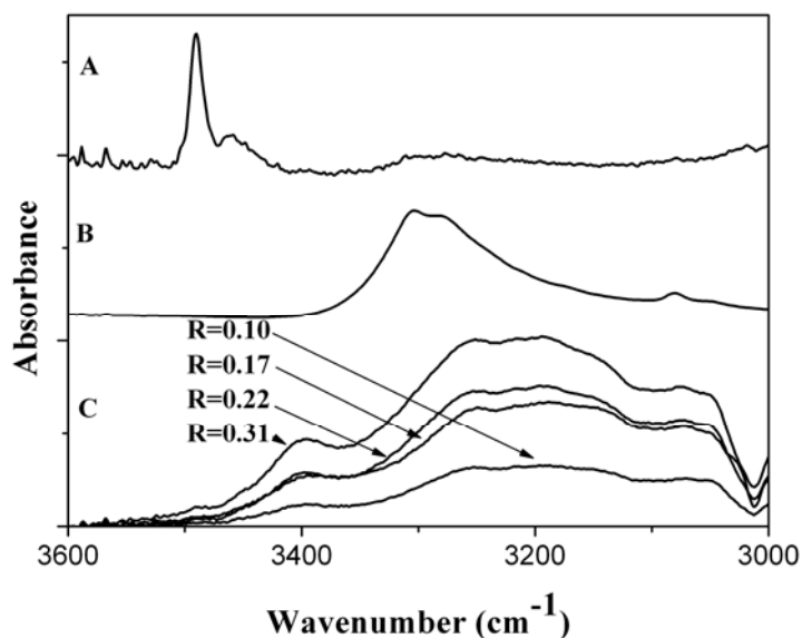
Figure 5. Comparison between IR spectra of MLT dispersed in CCl 4 (A), pure MLT (B) and MLT/lecithin/CCl 4 system at various R values (C).
