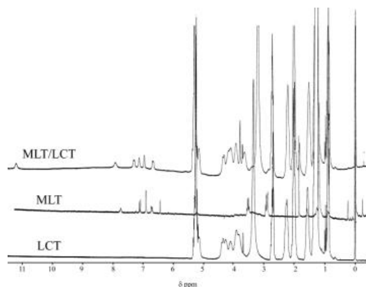
Figure 2. Comparison between the 1 H-NMR ( \text{CCl}_4 ) spectra of MLT, MLT/LCT ( R=0.31 ) and that of LCT systems.
