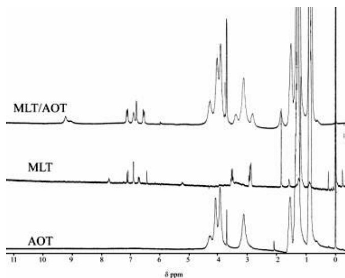
Figure 7. Comparison between the ^1\text{H-NMR} ( \text{CCl}_4 ) spectra of MLT, MLT/AOT ( R=0.18 ) and that of AOT systems.
