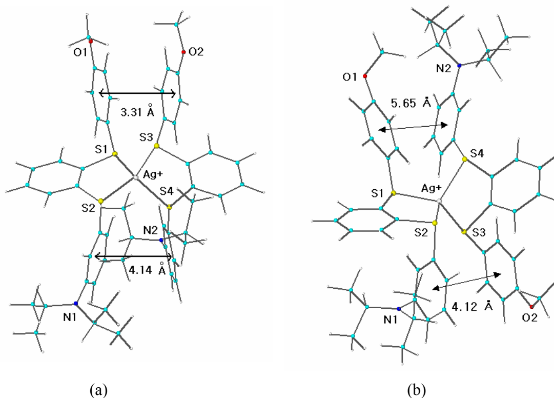
Figure 3. Molecular mechanics-calculated conformations of (a) 13a (parallel) – Ag + and (b) 13a (anti-parallel) – Ag + picrate complexes.
