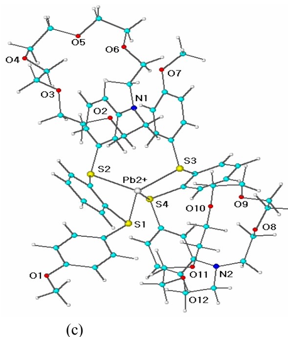
Figure 6. Molecular mechanics-calculated conformations of (a) the uncoordinated ligand 7j , (b) the bent-type and (c) the sandwich-type 7j - \text{Pb}^{2+} picrate complexes.
