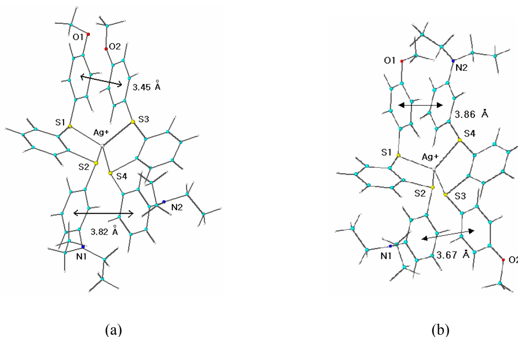
Figure 4. Molecular mechanics-calculated conformations of (a) 7a (parallel) – Ag + and (b) 7a (anti-parallel) – Ag + picrate complexes.
