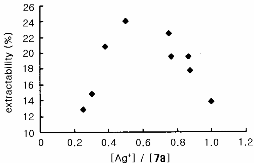
Figure 8. Extractability of 7a for Ag + ion versus the mole fraction [Ag + ]/[ 7a ].
