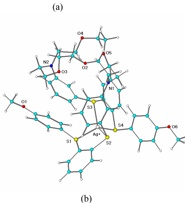
Figure 7. Molecular mechanics-calculated conformations of (a) the uncoordinated ligand 18a and (b) the 18a - Ag + picrate complex.
