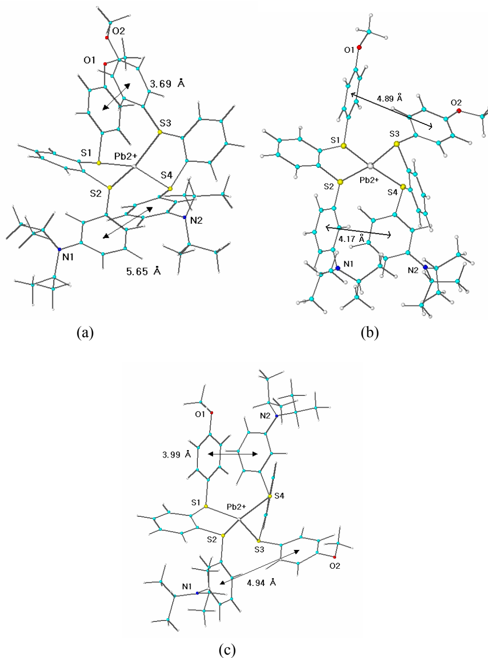
Figure 2. Molecular mechanics-calculated conformations of (a) 13a (parallel) – Pb 2+ , (b) 13a (parallel, T-shaped) – Pb 2+ , and (c) 13a (anti-parallel) - Pb 2+ picrate complexes.
