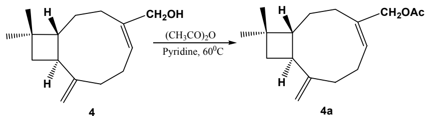
Scheme 3. Acetylation of 14-hydroxy-isocaryophyllene ( 4 ).
