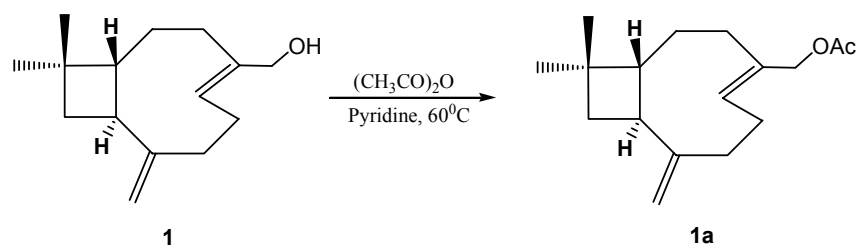
Scheme 1. Acetylation of 14-hydroxy- \beta -caryophyllene ( 1 ).
