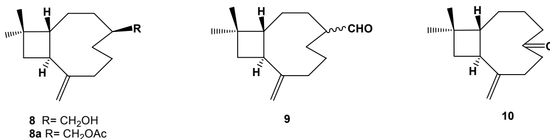
Figure 1. Isolated and semi-synthetic new compounds from B. litwinowii .
