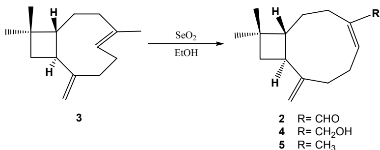
Scheme 2. Oxidation of \beta -caryophyllene ( 3 ).
