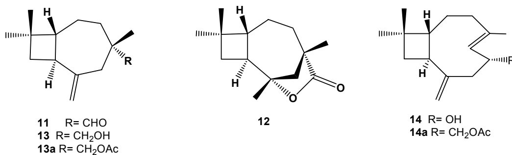
Figure 2. Isolated and semi-synthetic compounds from Betula pubescens .
