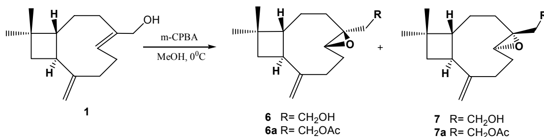
Scheme 4. Epoxidation of 14-hydroxy-β-caryophyllene ( 1 ).
