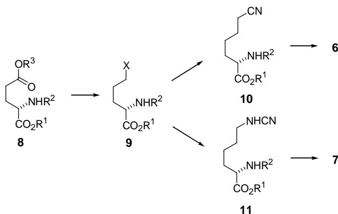
Scheme 1. Synthetic plan of L-NOHI ( 6 ) and L-homoNOHA ( 7 ) from the glutamate 8 .
