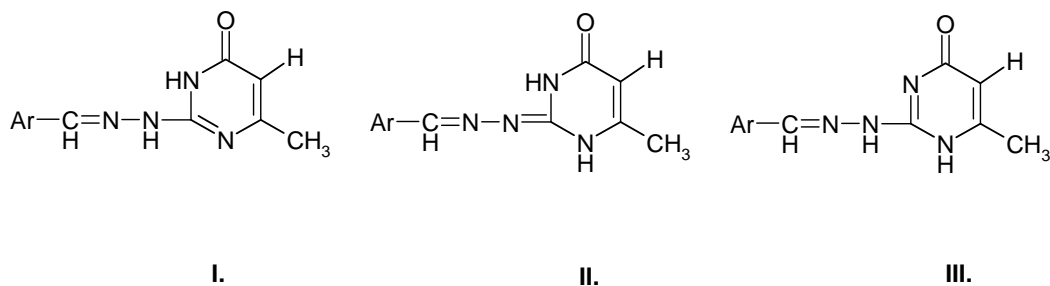
Scheme 2. Possible tautomers of arylidenehydrazones.
