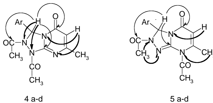
Scheme 4. Relevant ^{13}\text{C} - (thin lines) and ^{15}\text{N} -HMBC (thick lines) correlations.
