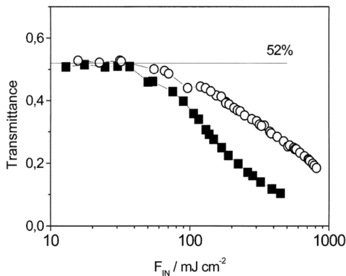
Figure 3. Non-linear transmittance of sh-SWNT-PEG (solid squares) and of suspended SWNT (open circles) in chloroform.
