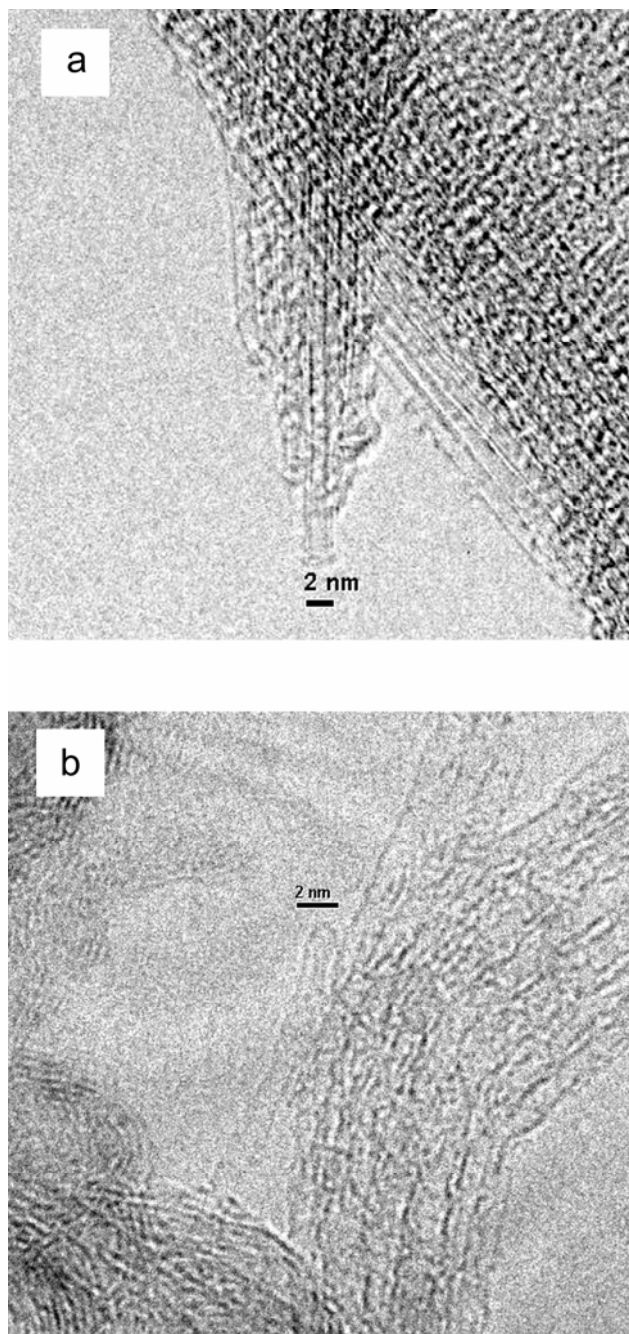
Figure 2. TEM images of a) sh-SWNTs (see text) and b) pristine SWNTs showing a single nanotube with the hemifullerene terminal cup at the center of the image.
