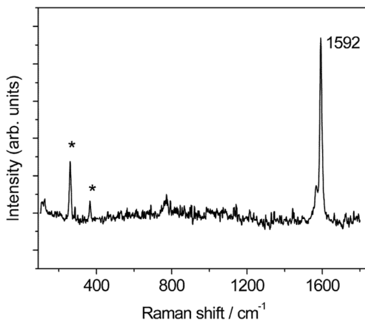
Figure 1. Raman spectrum (exciting line at 488 nm) of a solution of sh-SWNT-PEG in chloroform; the peaks labeled (*) are due to chloroform. The baseline was corrected for the luminescence background.
