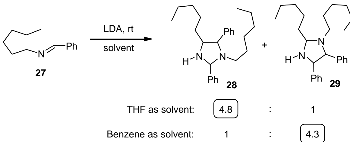
Scheme 7. Deliberate synthesis of imidazolidines from a 2-azaallyllithium.
