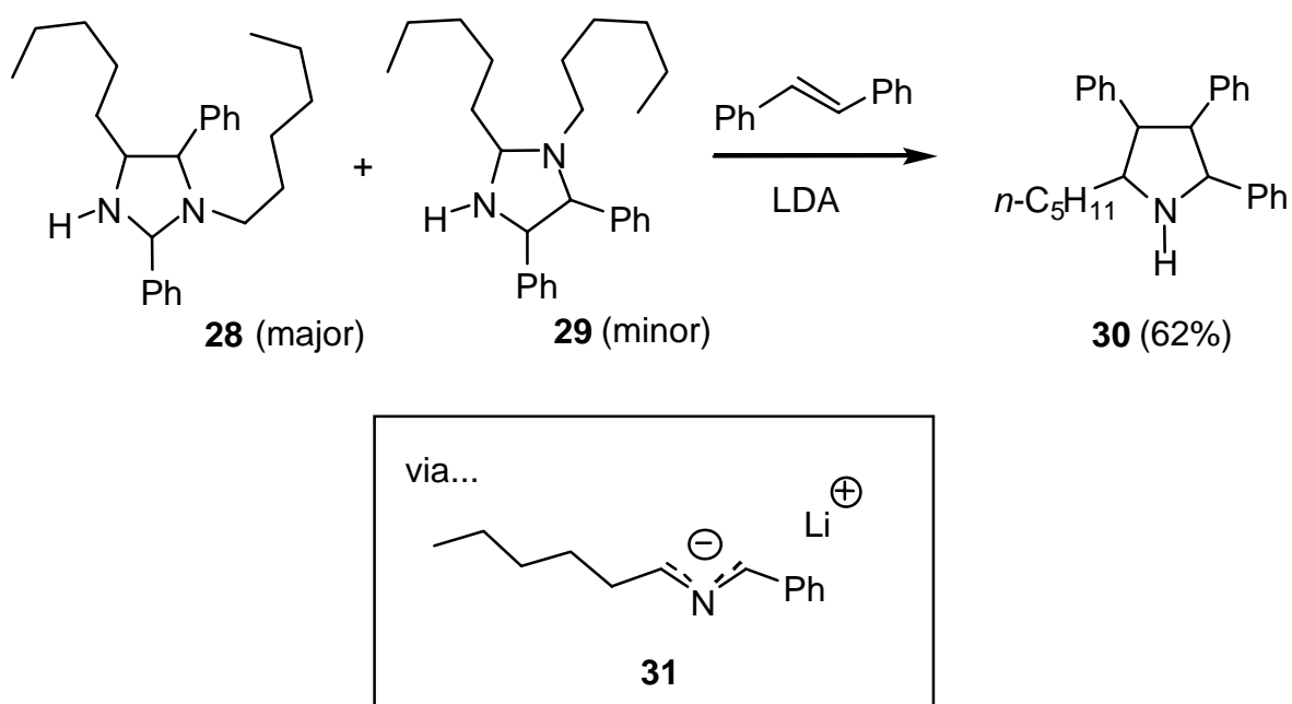
Scheme 8. Cycloreversion of imidazolidines and intermolecular cycloaddition of the resultant 2-azaallyllithium.
