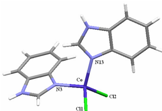
Figure 1. Dichloro-bis(1 H -benzimidazole)-cobalt(II). 18a
