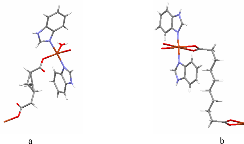
Figure 11. (a) Catena -(( \mu_2 -trans-2-butene-1,4-dicarboxylato- O,O',O'',O''' )-aqua-bis(1 H -benzimidazole)-copper(II)).; (b) catena -[( \mu_2 -octane-1,8-dicarboxylato- O,O',O'',O''' )-bis(1 H -benzimidazole)-copper(II)]. 29a, 29c
